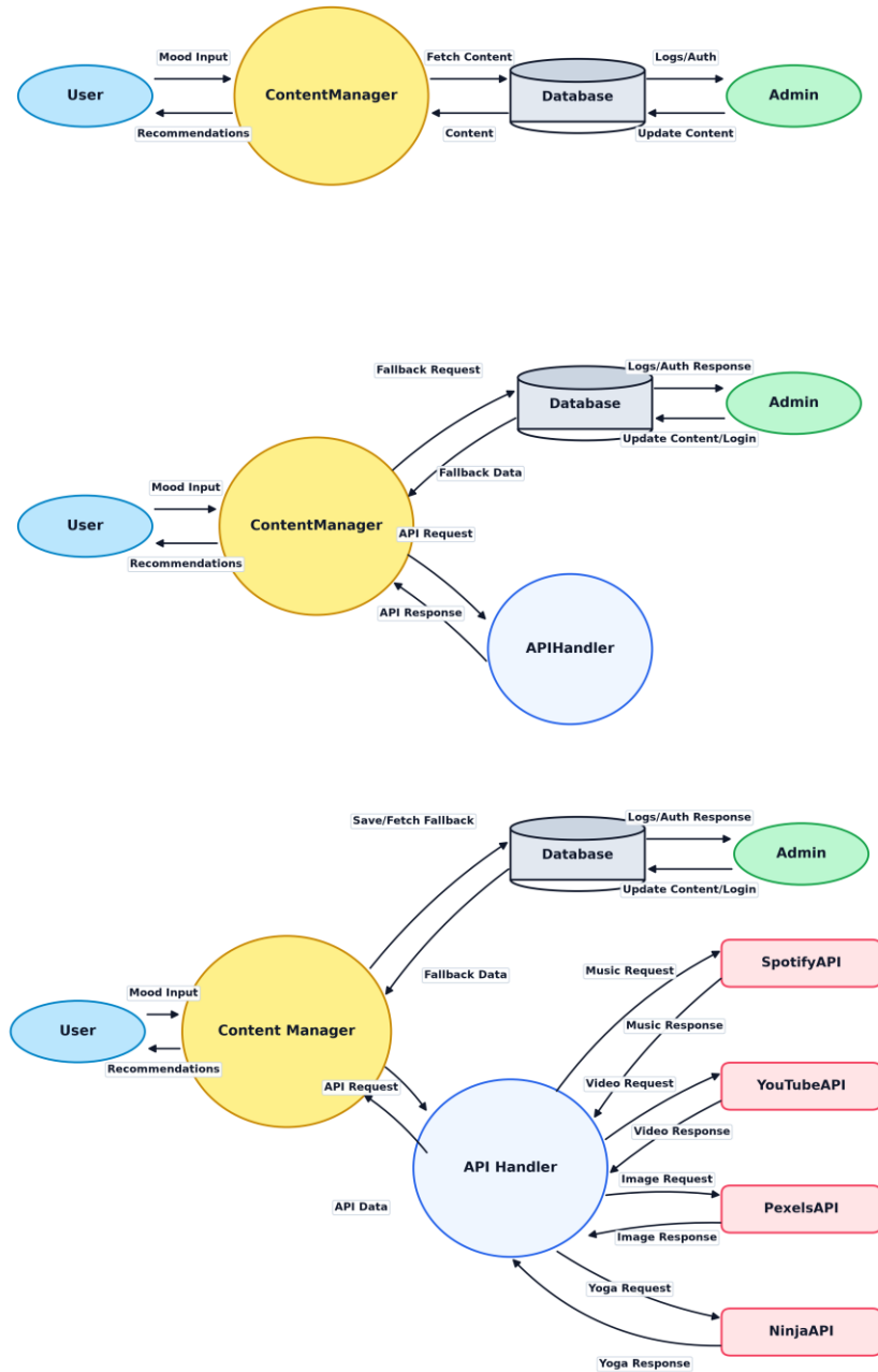
Figure 8.5 Data Flow Diagram
