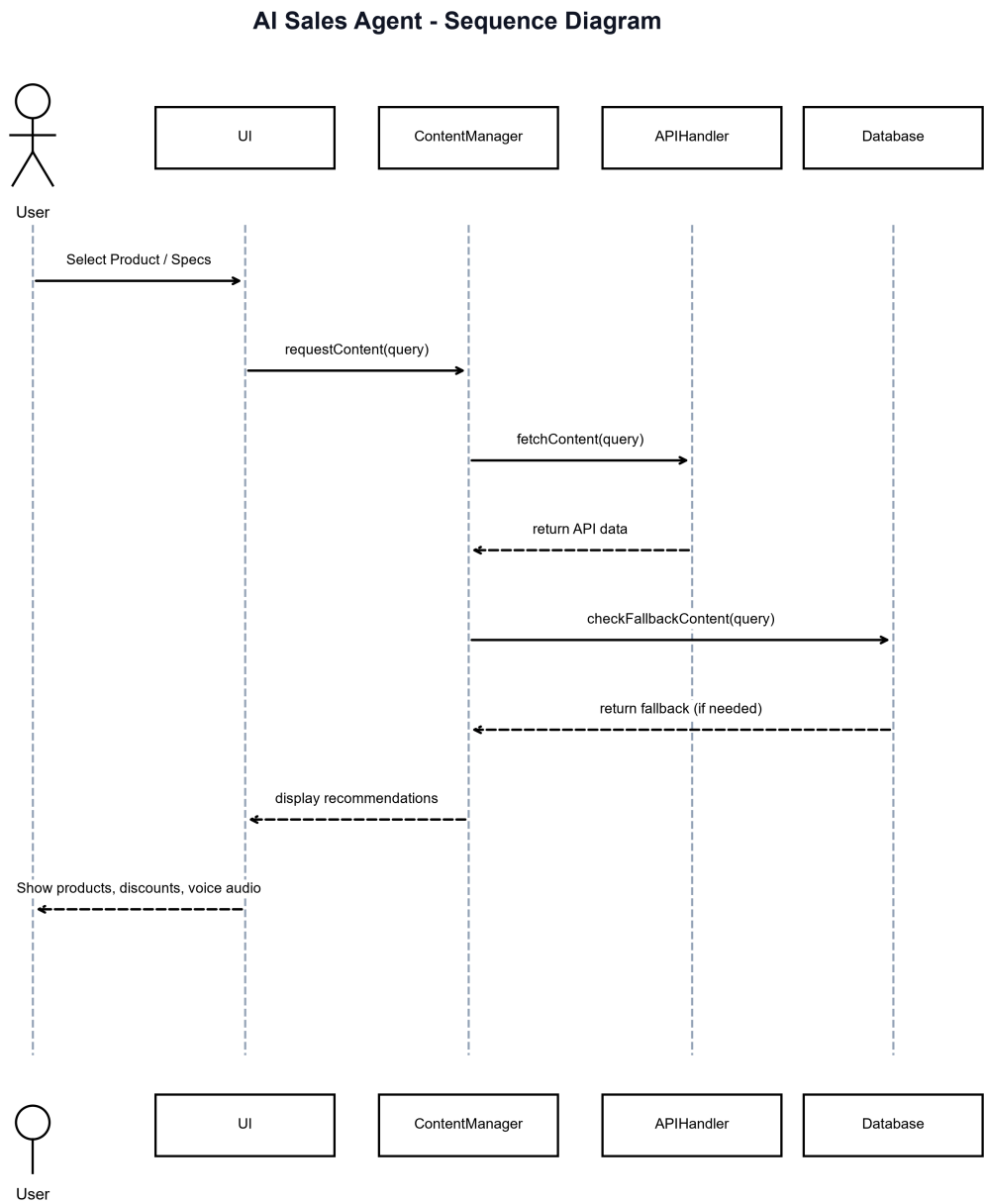
FIGURE 8.3 SEQUENCE DIAGRAM
