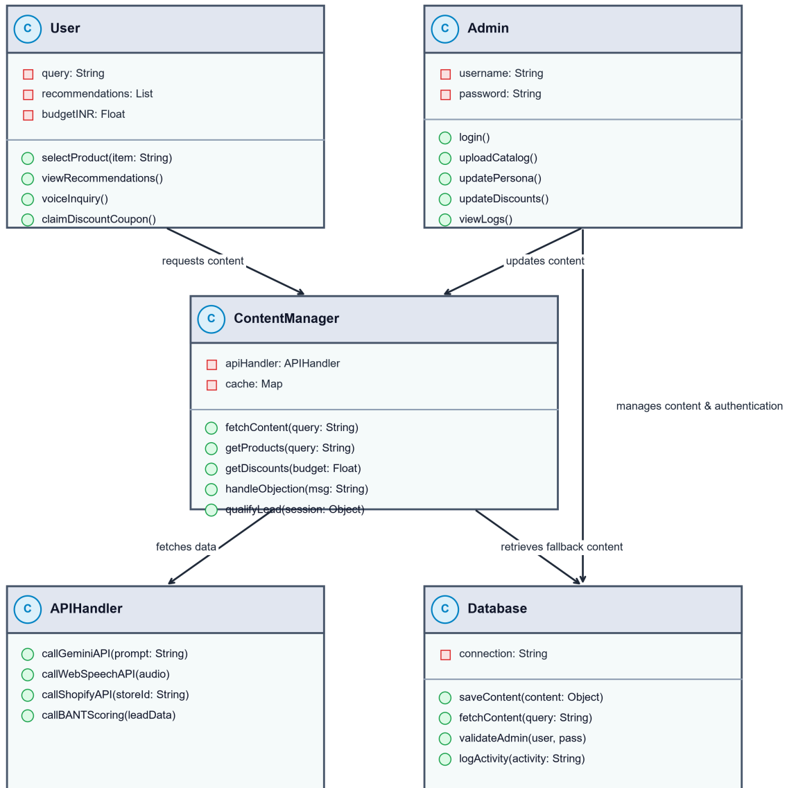
AI Sales Agent - Class Diagram
