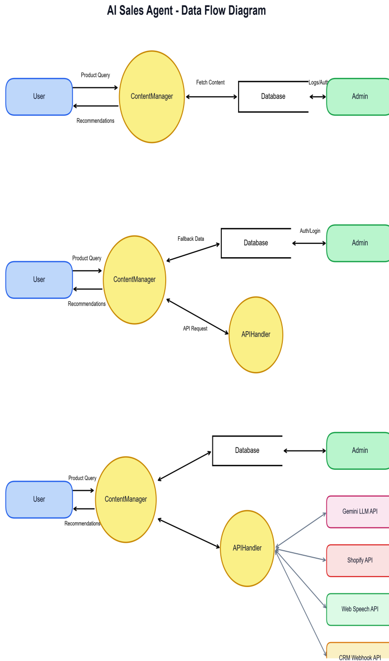
Figure 8.5 Data Flow Diagram
