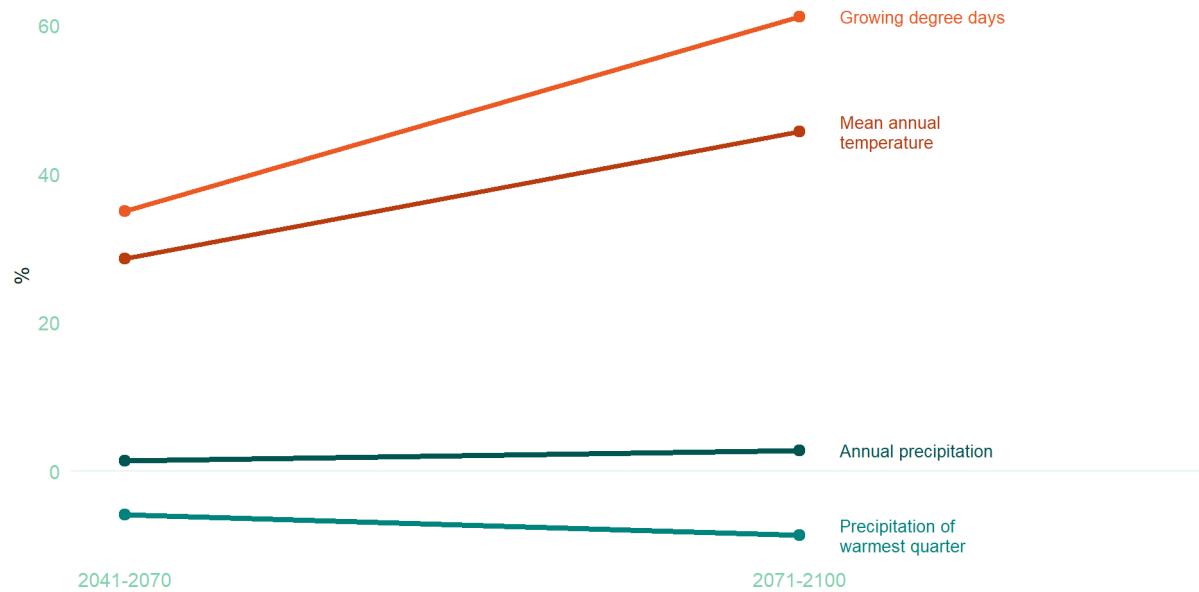
Figure 4: Chart showing Climate in the Hessian Low Mountain Range Living Lab (Data: Climate (CHELSA V2.1 / CMIP6): Growing degree days, Mean annual temperature, Annual precipitation, Precipitation of warmest quarter)
