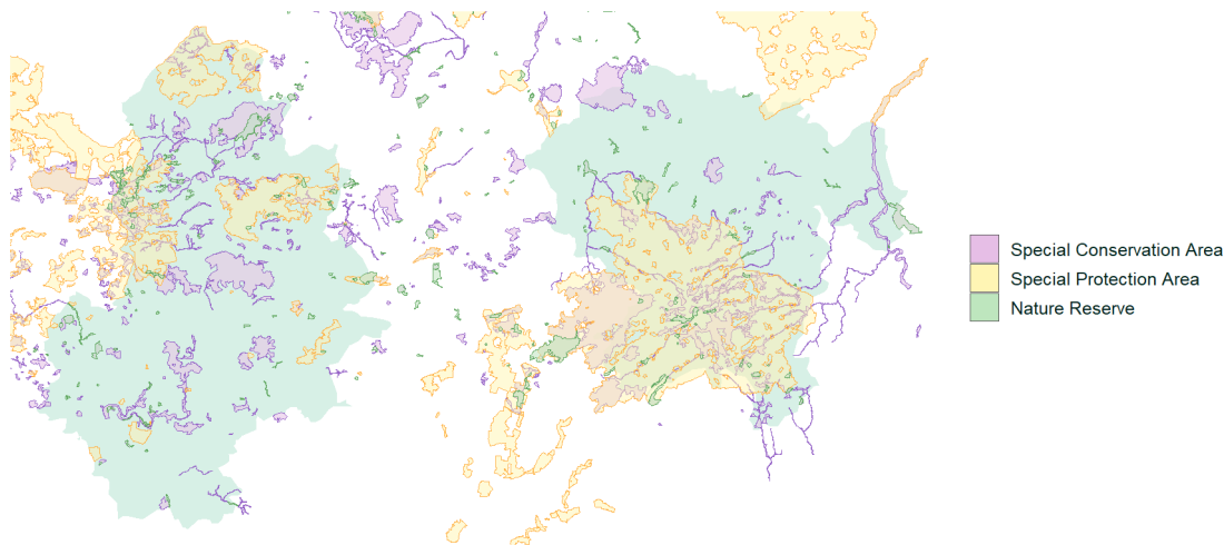
Figure 9: Map showing Protected Areas in the Hessian Low Mountain Range Living Lab (Data: Protected areas (BfN, 2019/2023))
