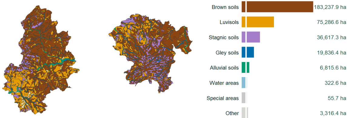
Figure 5: Map showing Soil in the Hessian Low Mountain Range Living Lab (Data: Soil overview map (BUEK250)) Legend shows the dominant semantic soil groups for this Living Lab; raw BUEK IDs stay in the data only as provenance.
