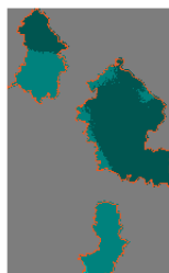
Summer precip. 2071-2100
