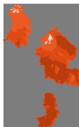
Precipitation Baseline
