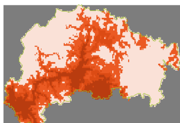
Precipitation Baseline
