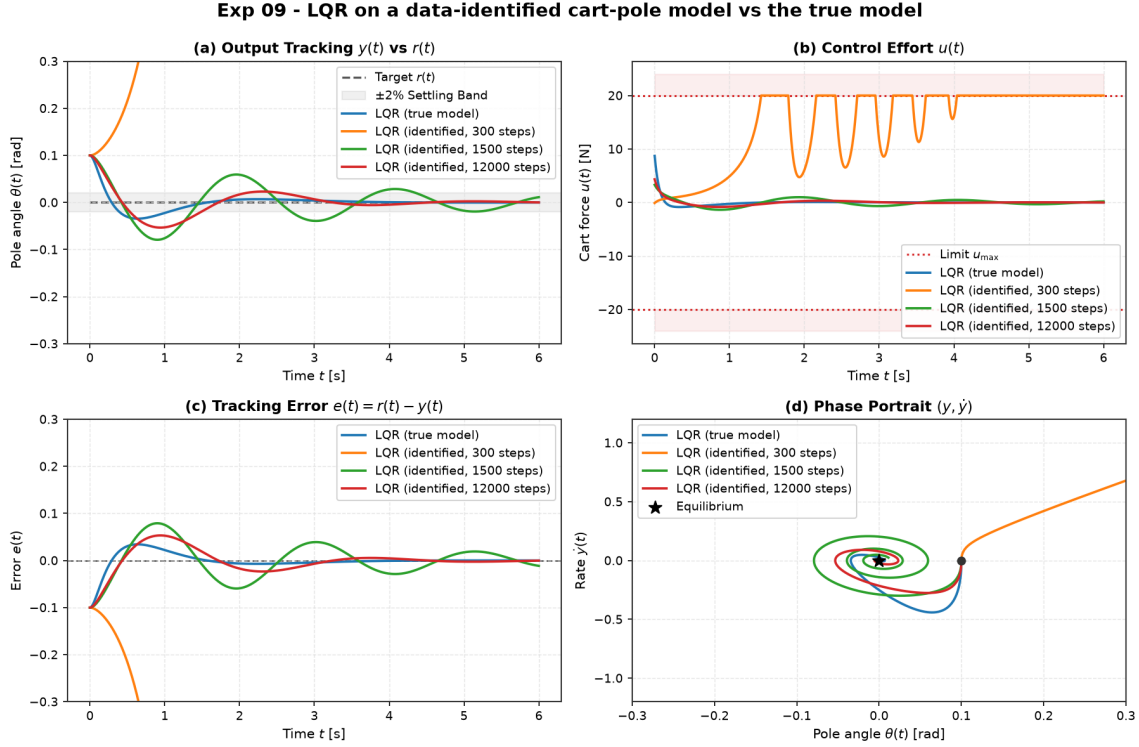
Figure 9: Experiment 09 benchmark comparison showing LQR performance designed on identified models from 300, 1500, and 12000 steps of training data versus true model baseline.
