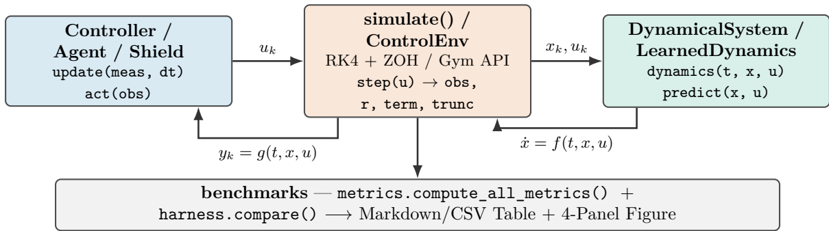
Figure 1: Core framework architecture. The numerical simulation engine drives a controller ( update() ) and continuous plant or learned neural surrogate ( dynamics() ) via fixed-step 4th-order Runge–Kutta with Zero-Order Hold (ZOH).
