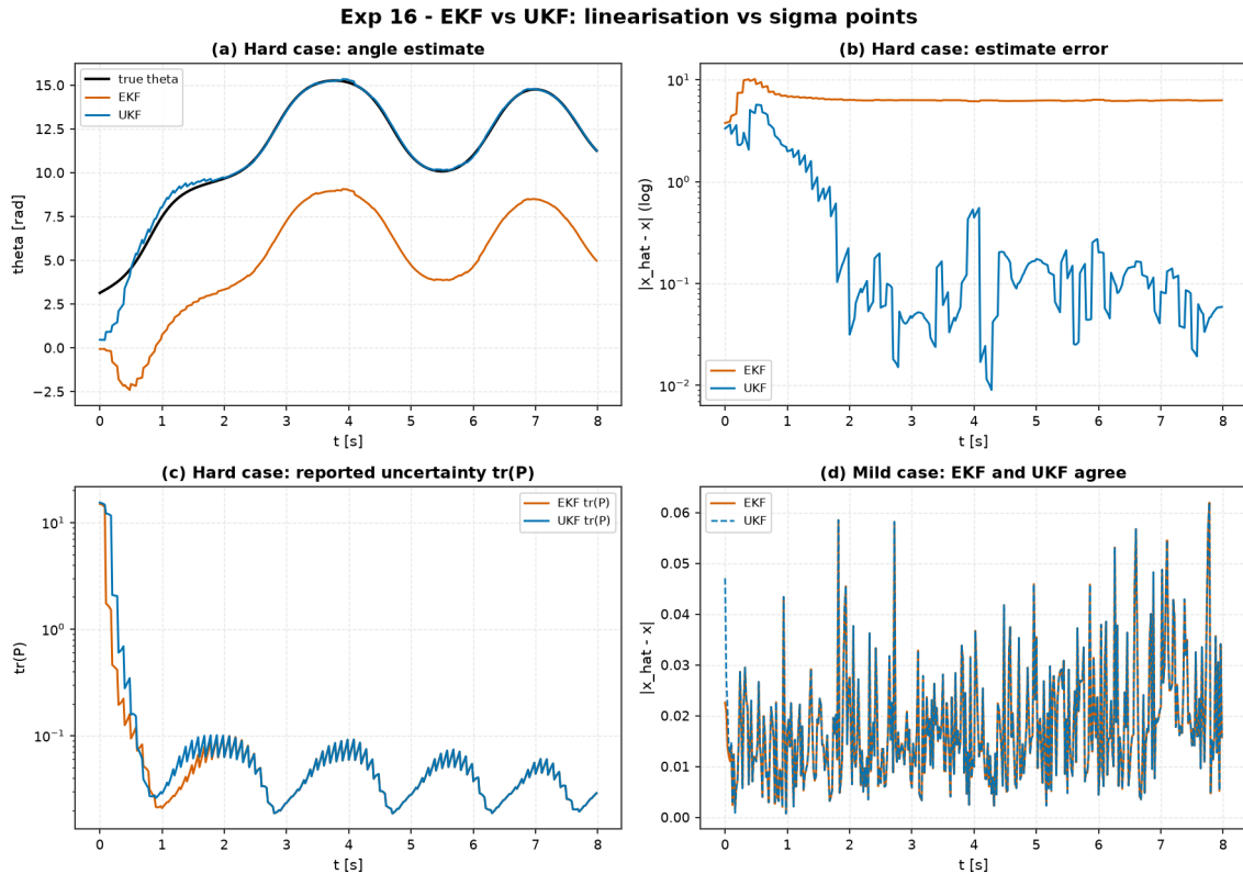
Figure 17: Experiment 16 benchmark comparison: EKF vs. UKF on nonlinear Pendulum estimation illustrating trajectory convergence, covariance trace \text{tr}(P) , and error profiles across hard and mild regimes.
