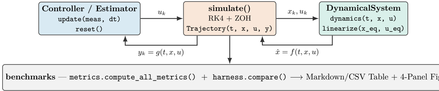
Figure 1: Core framework architecture. The numerical simulation engine drives a controller ( update() ) and continuous plant ( dynamics() ) via fixed-step 4th-order Runge–Kutta with Zero-Order Hold (ZOH). Optional hooks support custom sensor measurement transforms and additive input disturbances.
