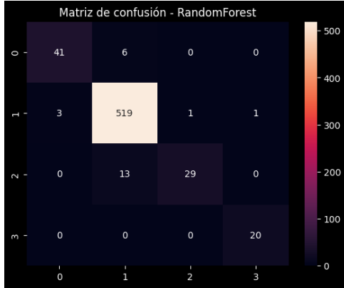
(a) RandomForest
