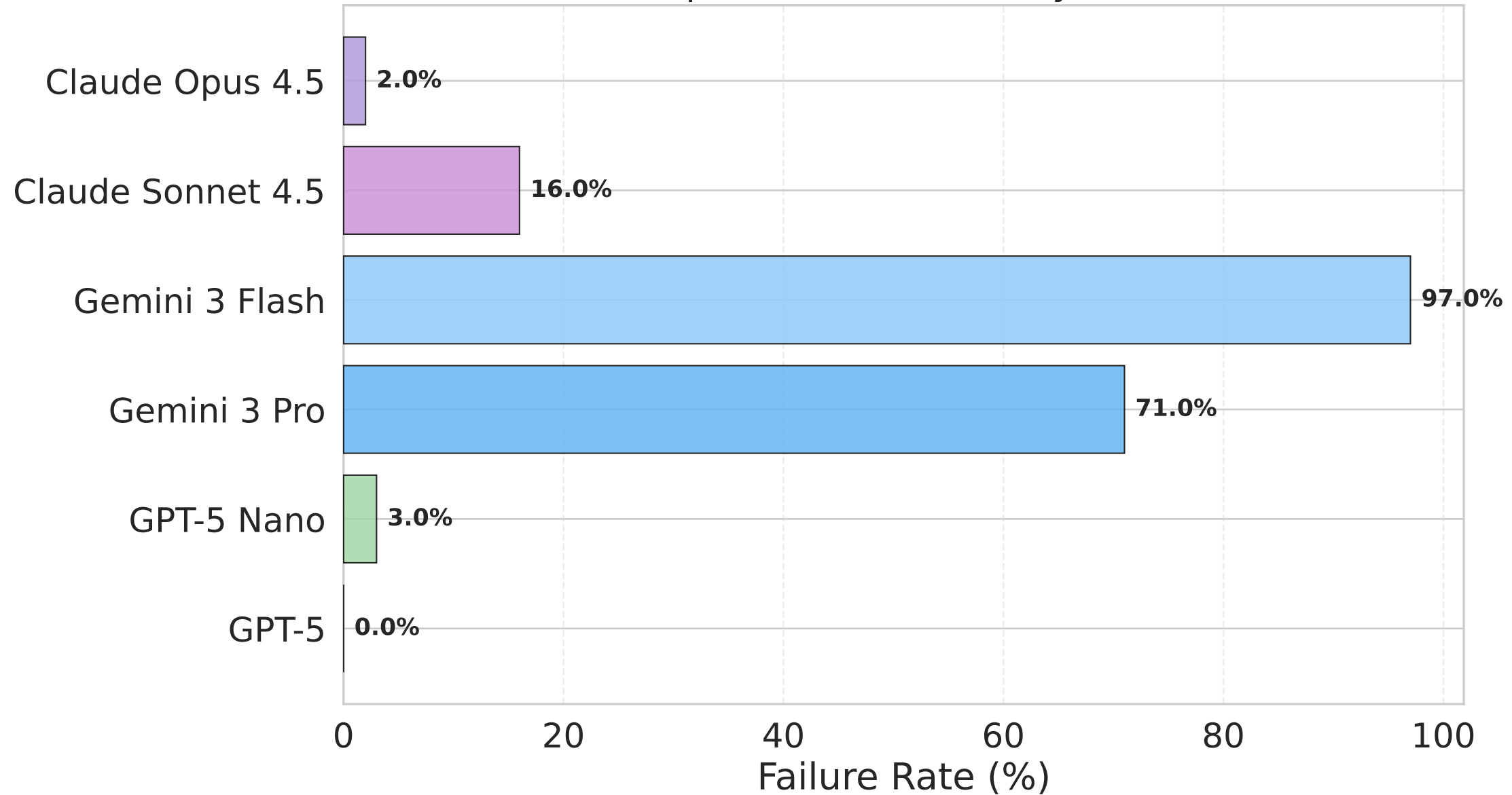
DeepEval Failure Rate by Model
