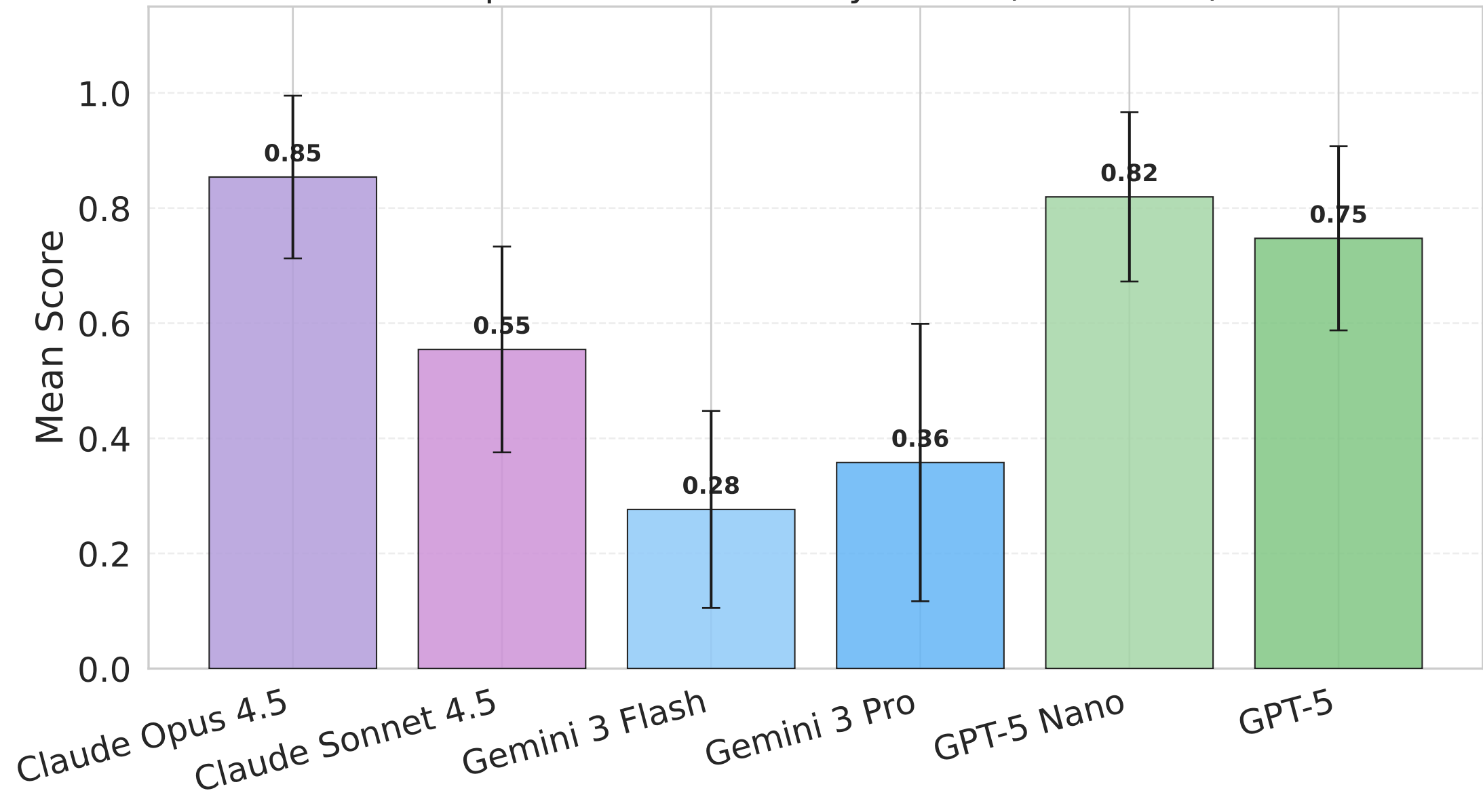
DeepEval Mean Score by Model ( \pm Std Dev)
