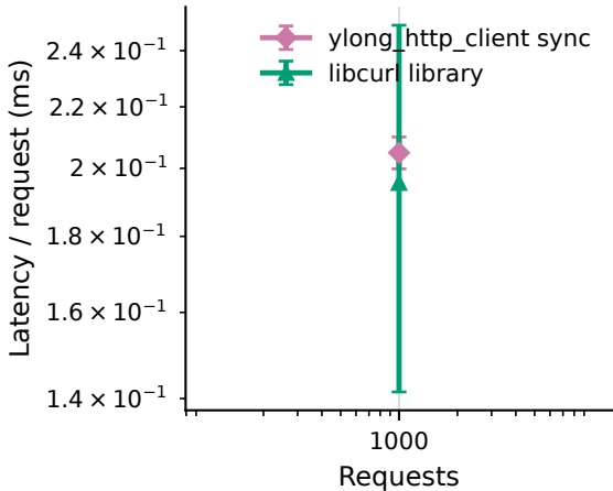
(a) Latency
