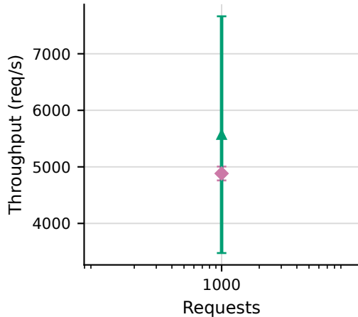
(b) Throughput
