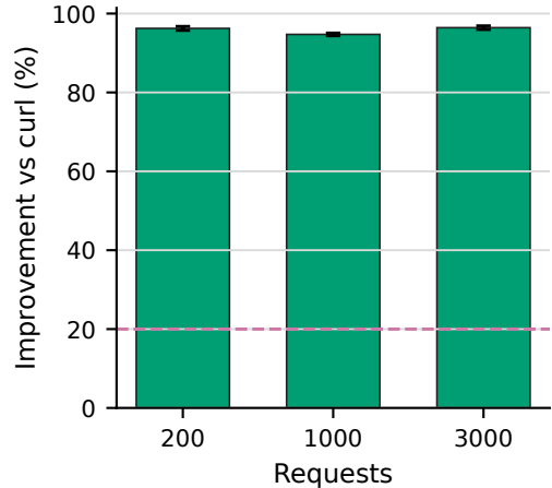
(c) Speedup margin
