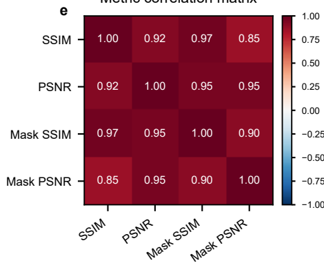
Metric correlation matrix
