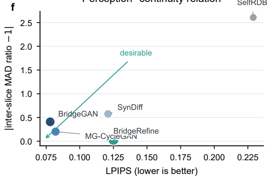
Perception--continuity relation
