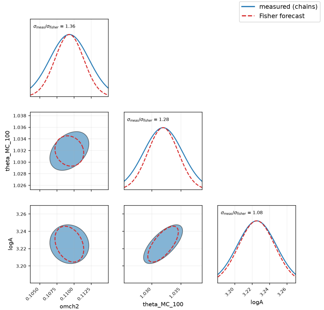
Figure 5: Triangle plot comparing the empirically found distributions and correlations with the Fisher forecast from the home-grown Fisher forecasting software in CMBLensing.py
