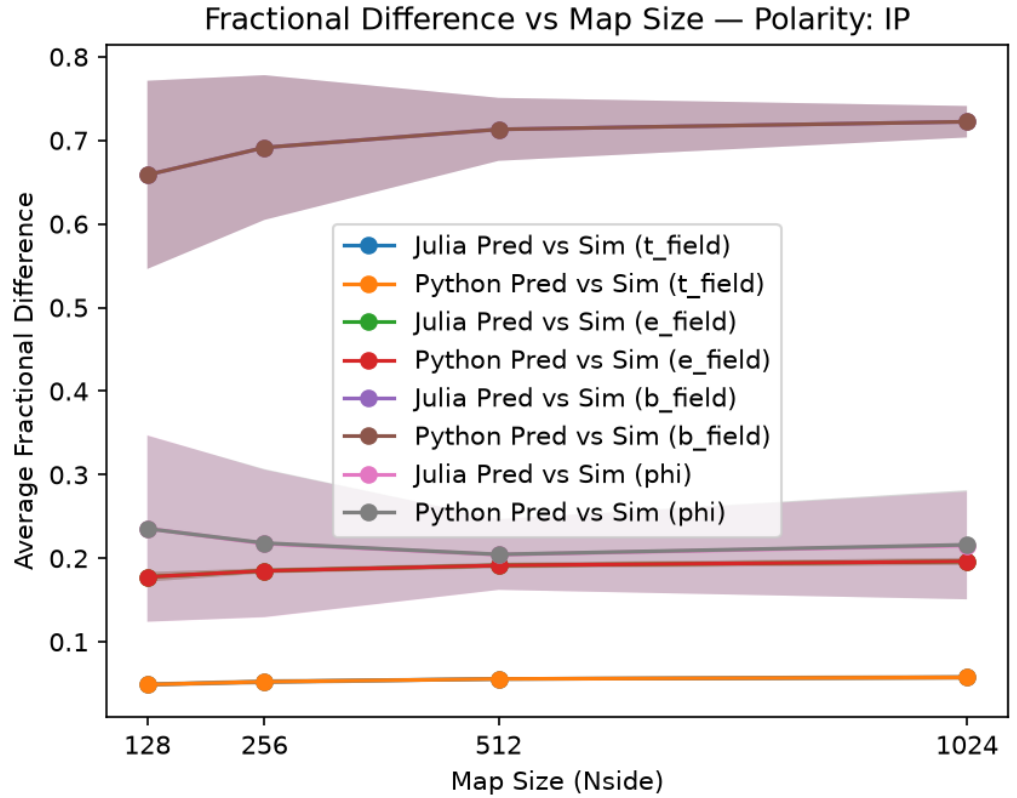
Figure 2: Fractional difference between the MAP estimates from either language and the simulation ground truth. Both use ground truth fields from the Julia simulation code, eliminating the possibility that the Python simulation and MAP code are wrong in a self-consistent way.
