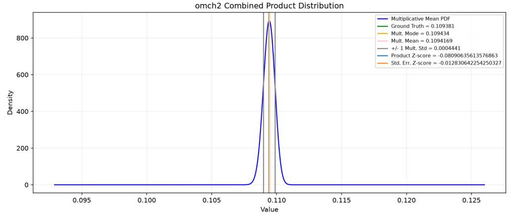
Figure 4: The resulting \Omega_c h^2 product distribution from 50 temperature data map realizations.
