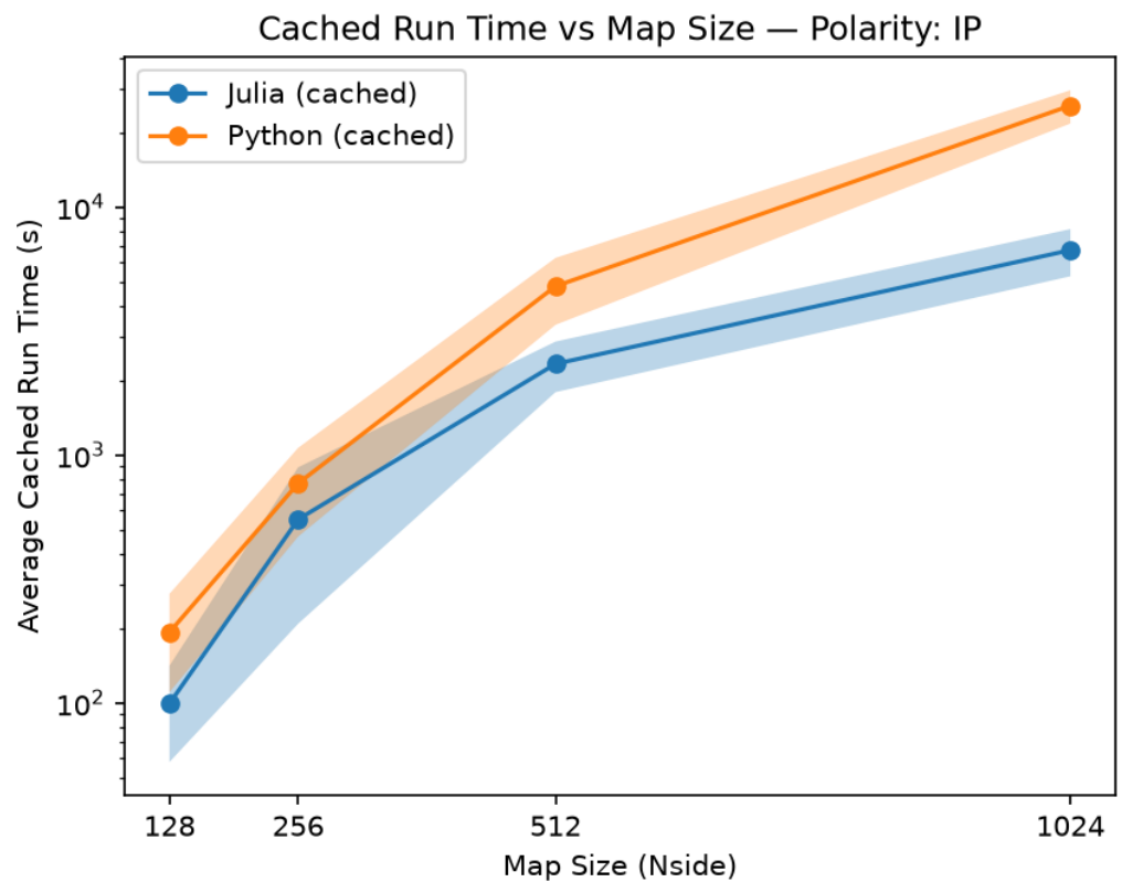
Figure 1: Run time comparison between language implementations of map_joint . The method is run twice in each language and the cached time is stored on the second call.
