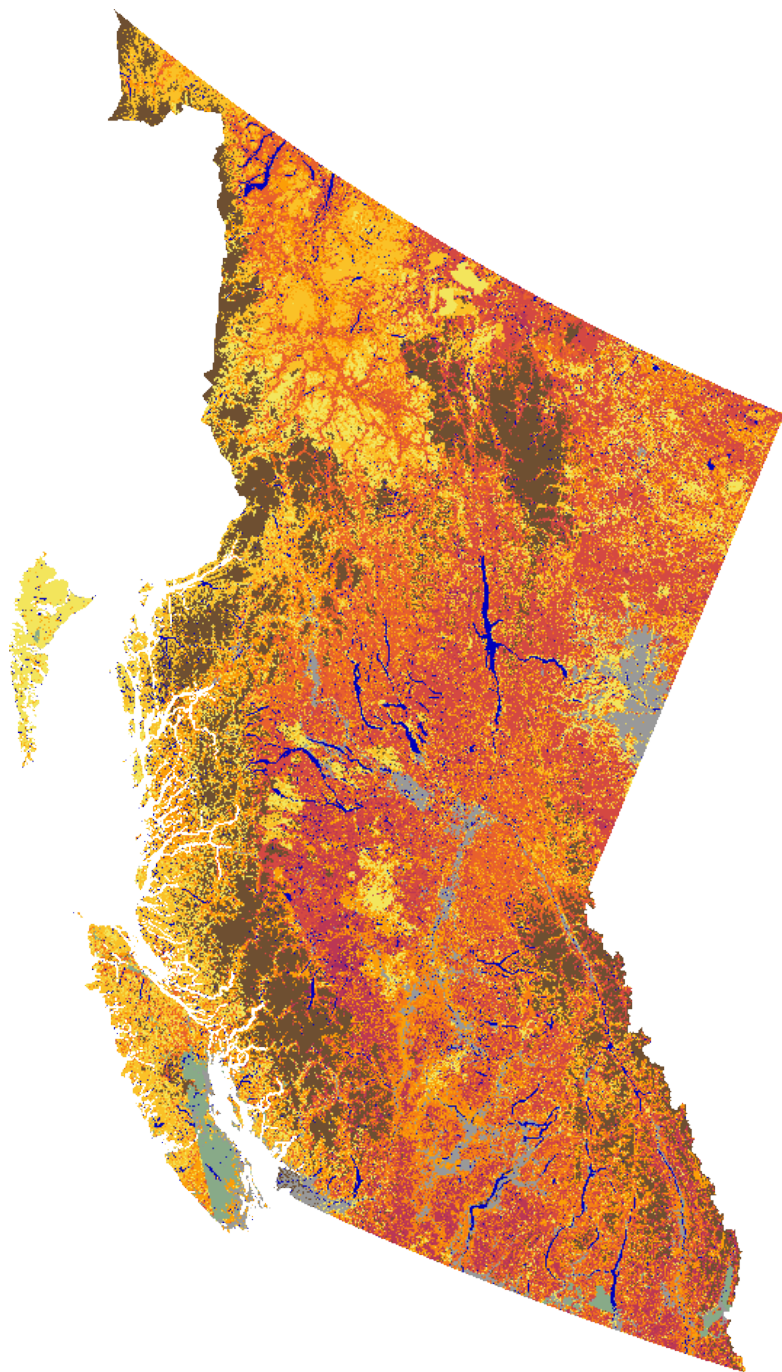
Head Fire Intensity (kW/m)
