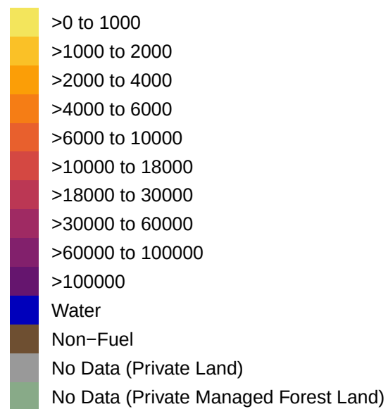
Head Fire Intensity (kW/m)
