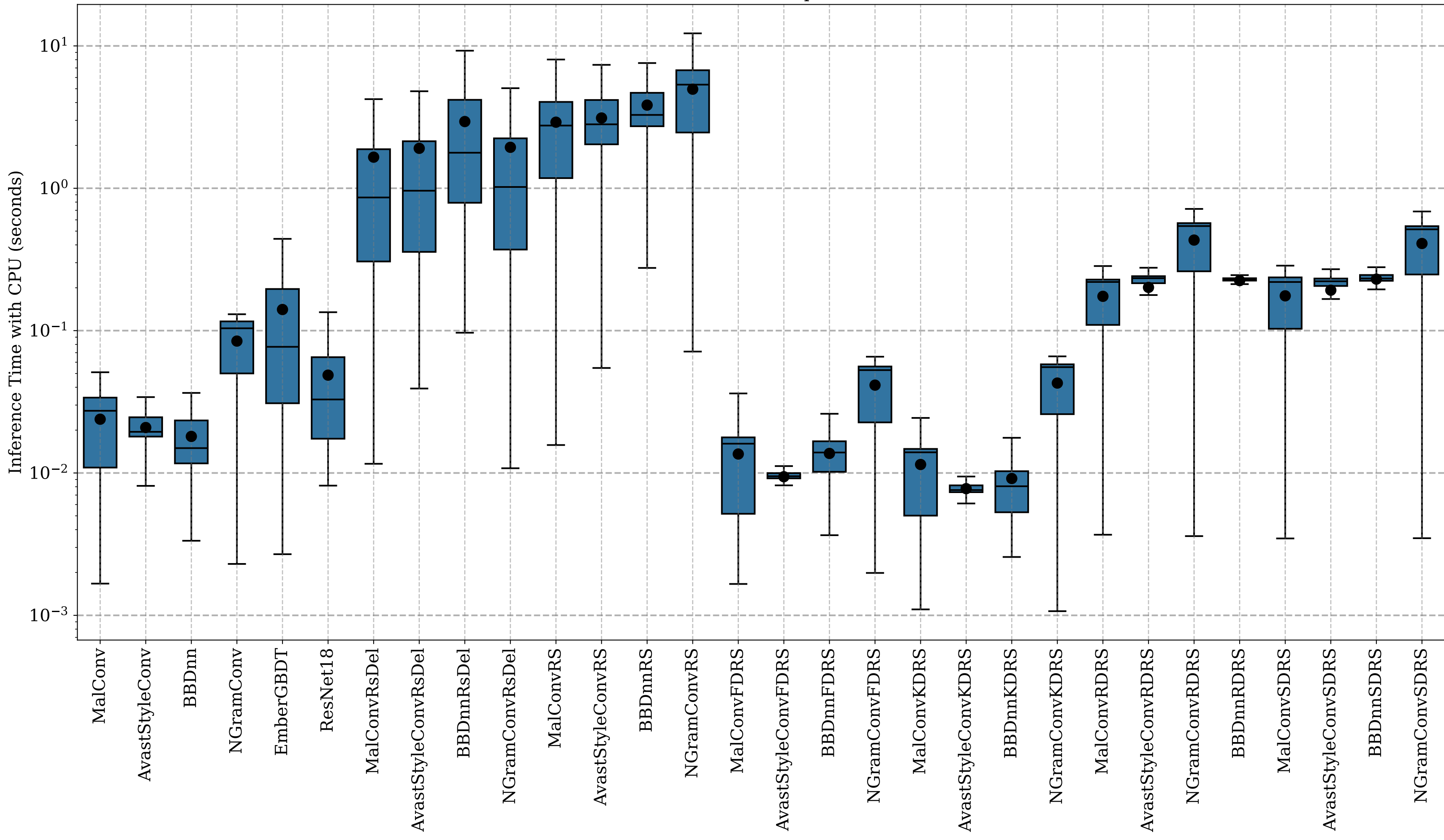
Inference Time Distribution per Model on CPU
