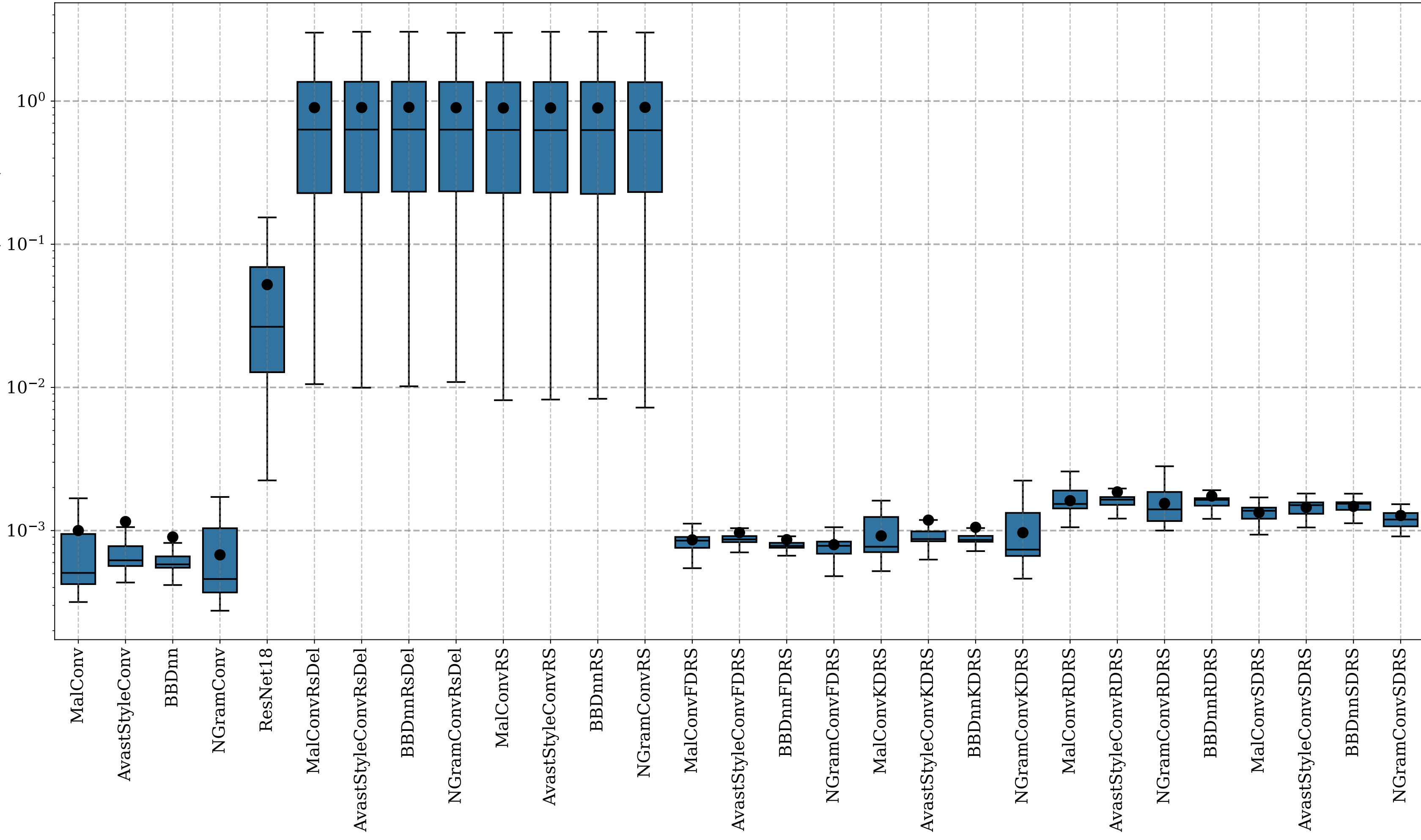
Inference Time Distribution per Model on GPU
