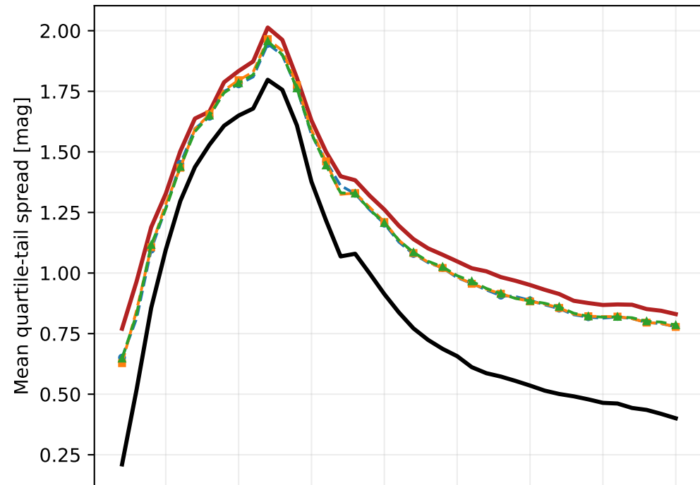
JWST F070W - F200W vs. F200W
