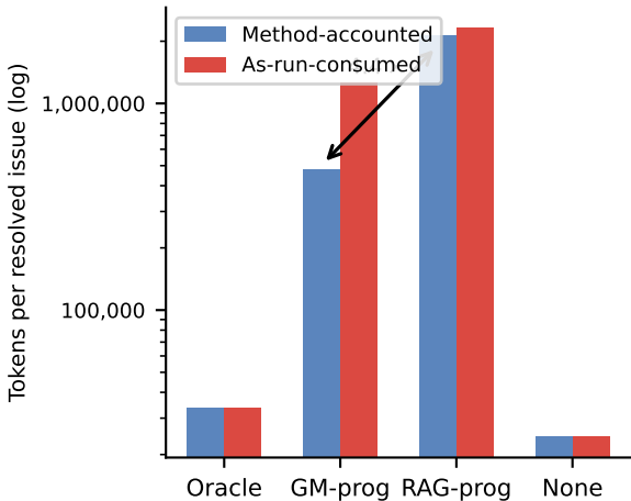
Cost per Resolved Issue
