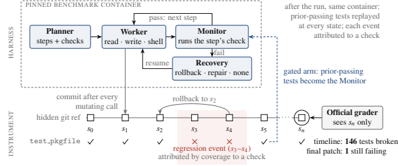
Figure 1: The harness and the instrument. The test row shows a previously-passing test regressing at s_3 – s_4 and repaired by a rollback to s_2 , which the official grader, reading only s_n , never sees. The counts are the GPT-5.6 rollback arm’s, over all 47 of its runs.
