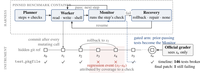
Figure 1: The harness and the instrument. The test row shows a previously-passing test regressing at s_3 – s_4 and repaired by a rollback to s_2 , which the official grader, reading only s_n , never sees. The counts are the GPT-5.6 rollback arm’s, over all 47 of its runs.
