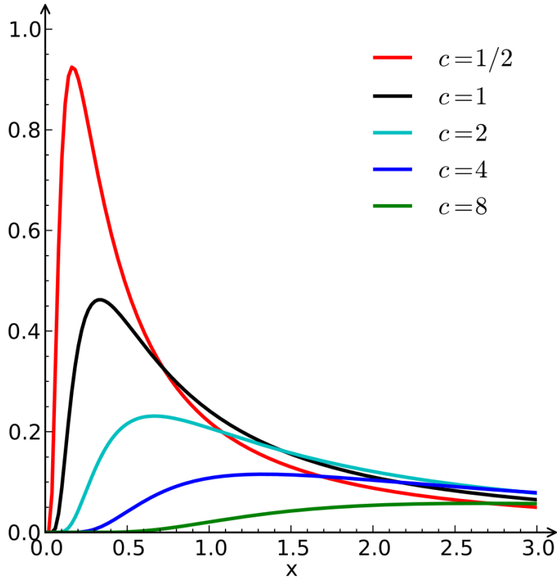
Figure 3.5: Probability densities of Lévy distributions for different parameter values [11].
