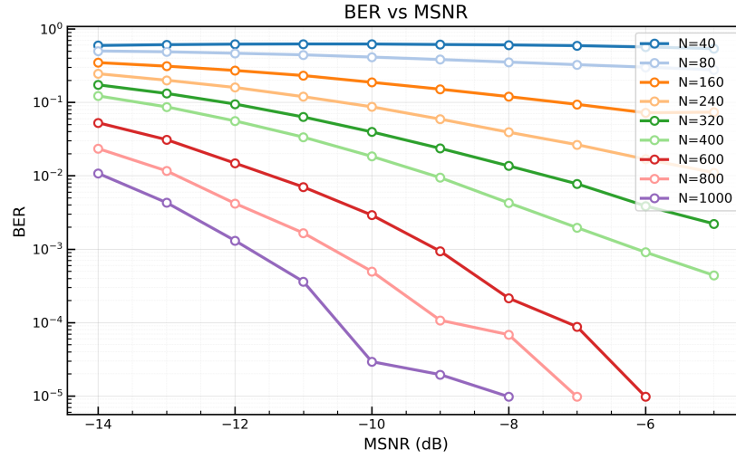
Figure 6.3: BER as a function of MSNR for different values of N .
