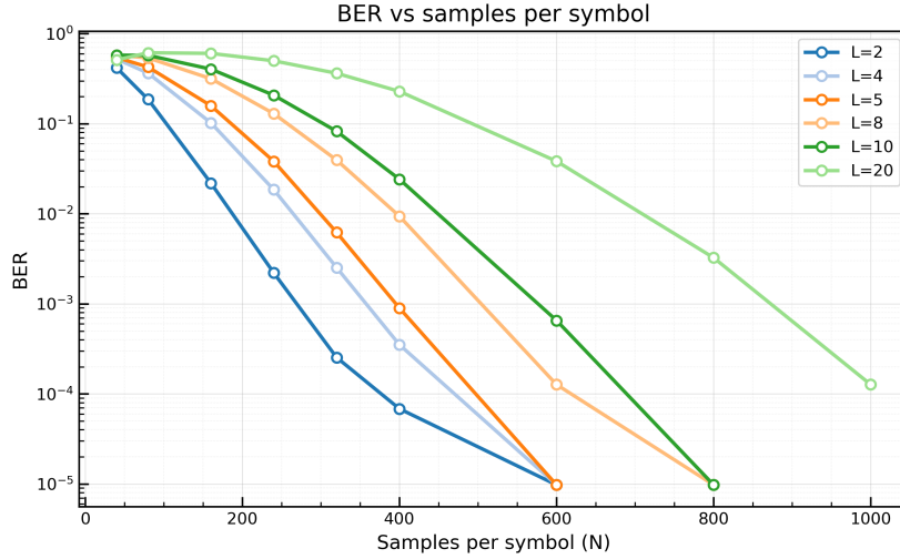
Figure 6.1: BER as a function of samples per symbol N for different values of L .
