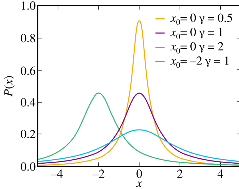
Figure 3.4: Probability densities of Cauchy distributions for different parameter values [10].
