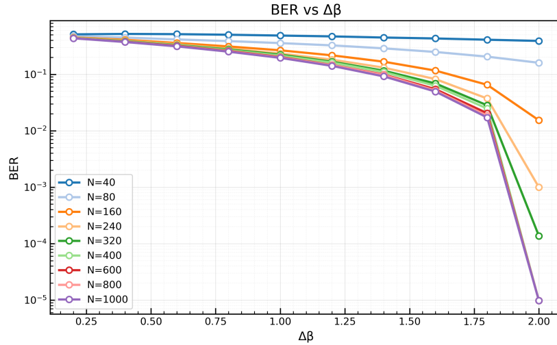
Figure 6.2: BER as a function of \Delta\beta for different values of N .
