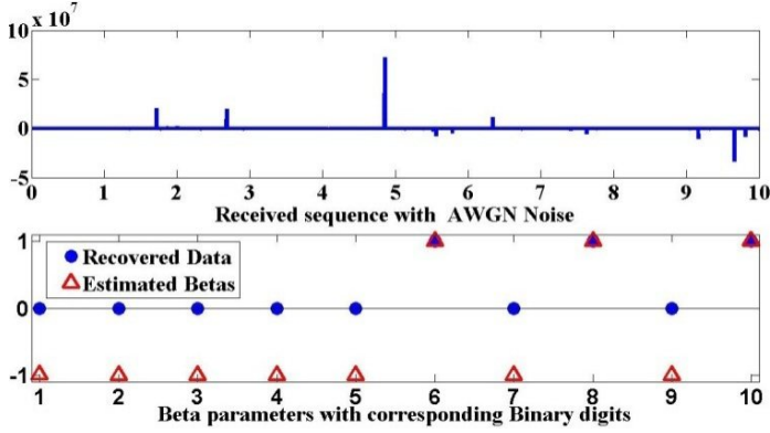
Fig. 3. Received signal from AWGN channel in time domain (Top), estimated beta parameters and recovered binary message (Bottom); bit length T_b = 1 , N = 1000 noise samples per information bit, T_b N = 1 \times 10^3 .
