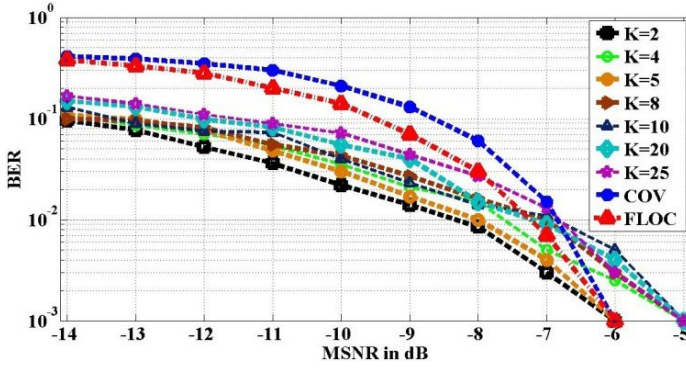
Fig. 4. BER versus MSNR (dB) with different “ L and K ” of estimator in AWGN channel; transmitted bits = 1000; where \alpha = 1.6 ; (where \beta_1 = -\beta_0 = 1 ).
