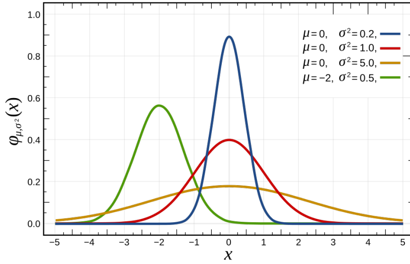
Figure 3.3: Probability densities of normal distributions for different parameter values [21].
