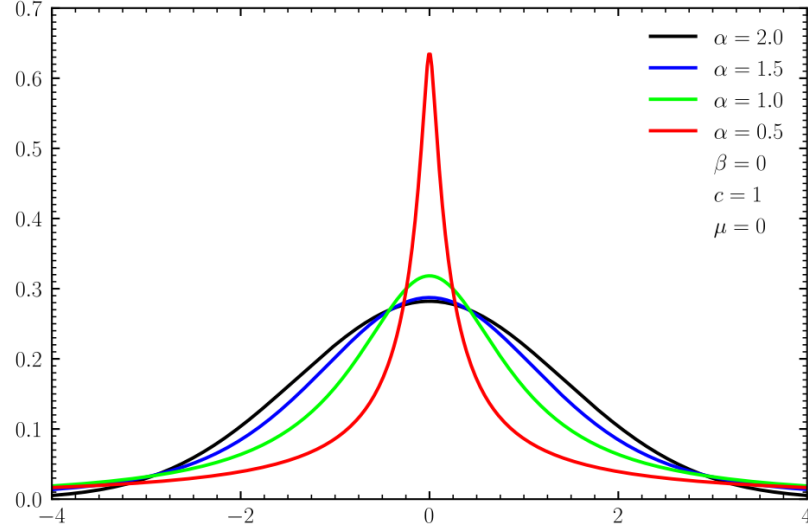
Figure 3.1: Distributions for different values of \alpha [22].
