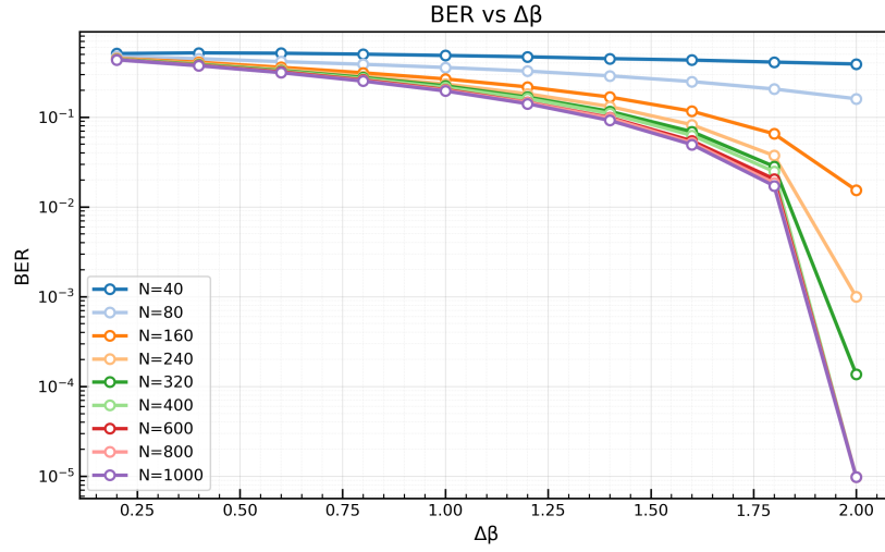
Figure 6.2: BER as a function of \Delta\beta for different values of N .
