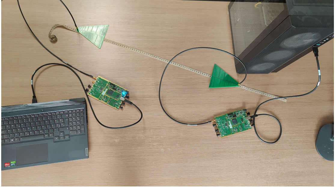
Figure 6.4: Experimental communication system comprising two USRP B210 devices, two WA5VJB LP8565A2 log-periodic antennas, and the transmitter and receiver computers.
