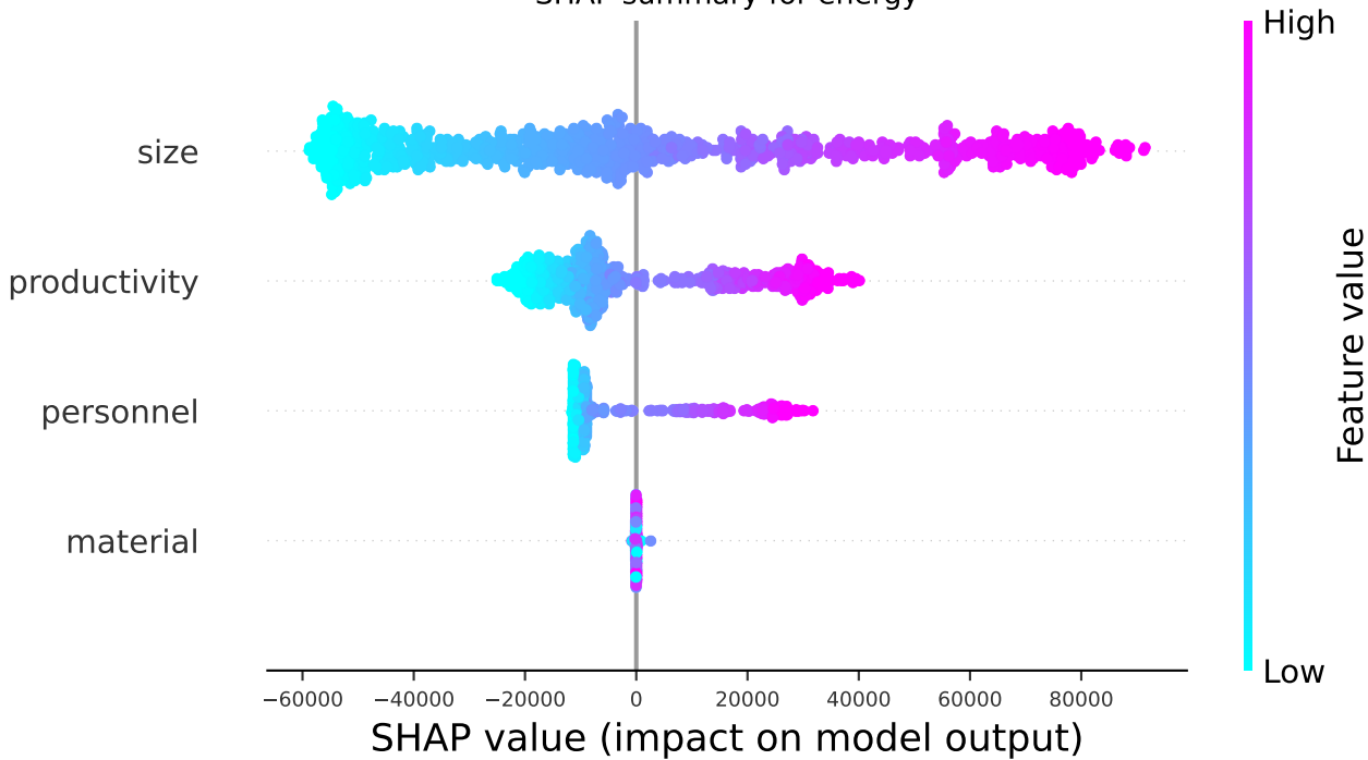
SHAP summary for energy
