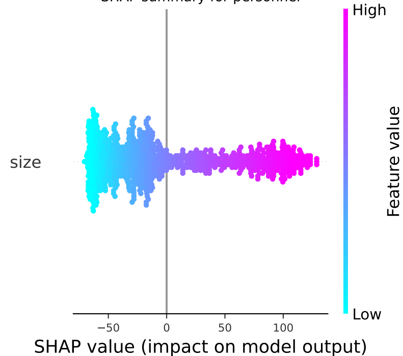
SHAP summary for personnel
