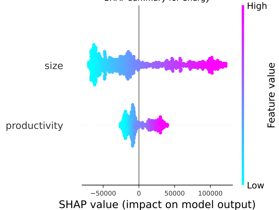
SHAP summary for energy
