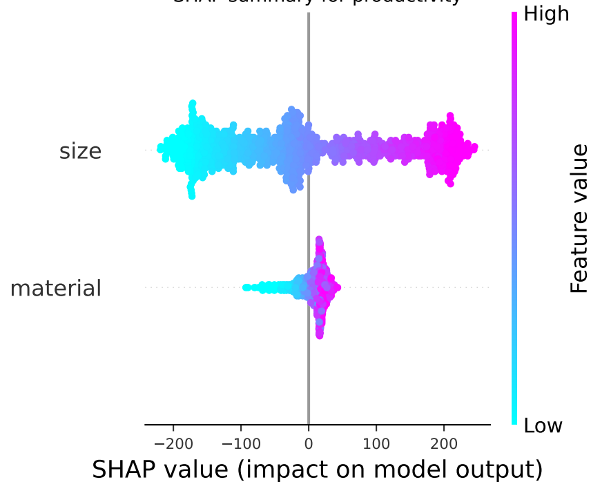
SHAP summary for productivity
