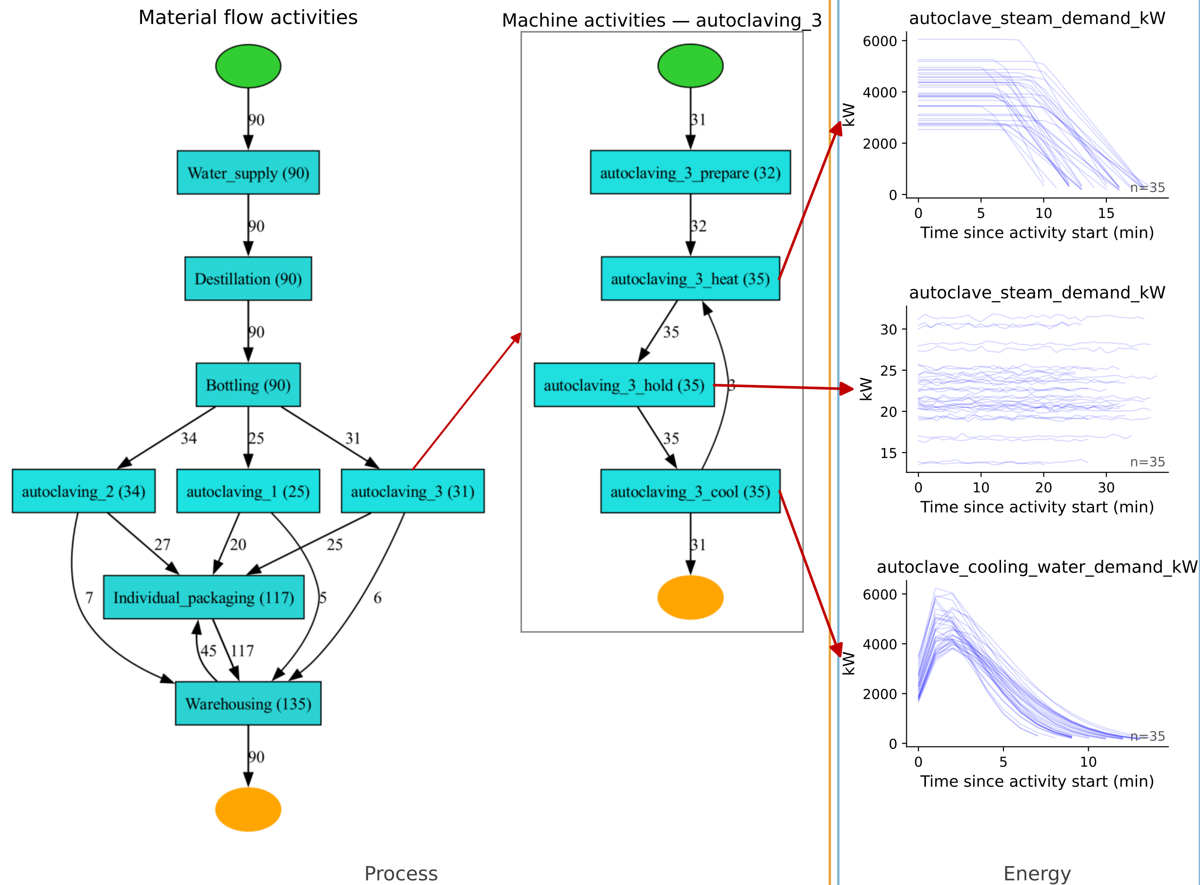
(a) real test set process and energy profiles
