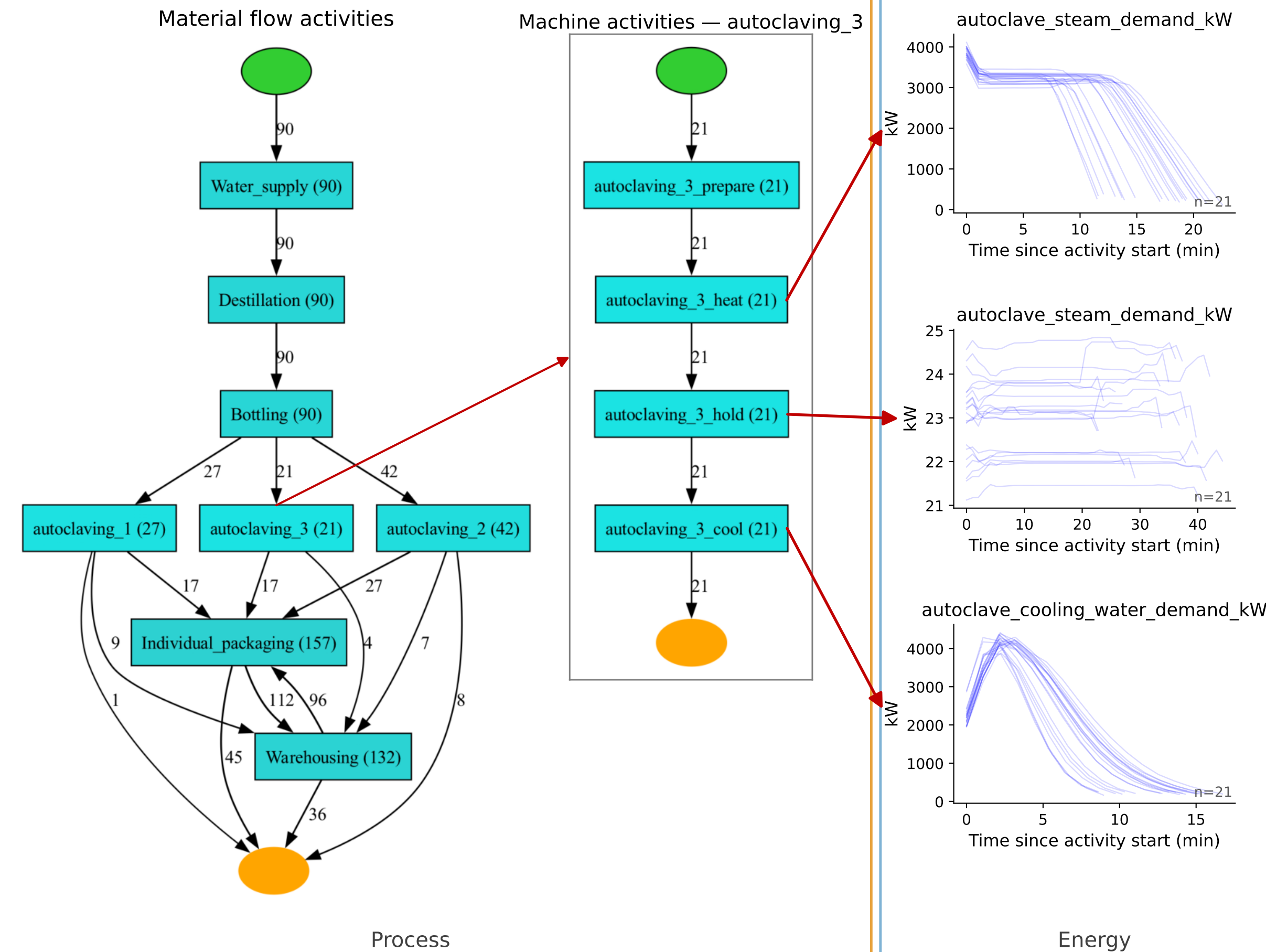
(b) simulated process and energy profiles
