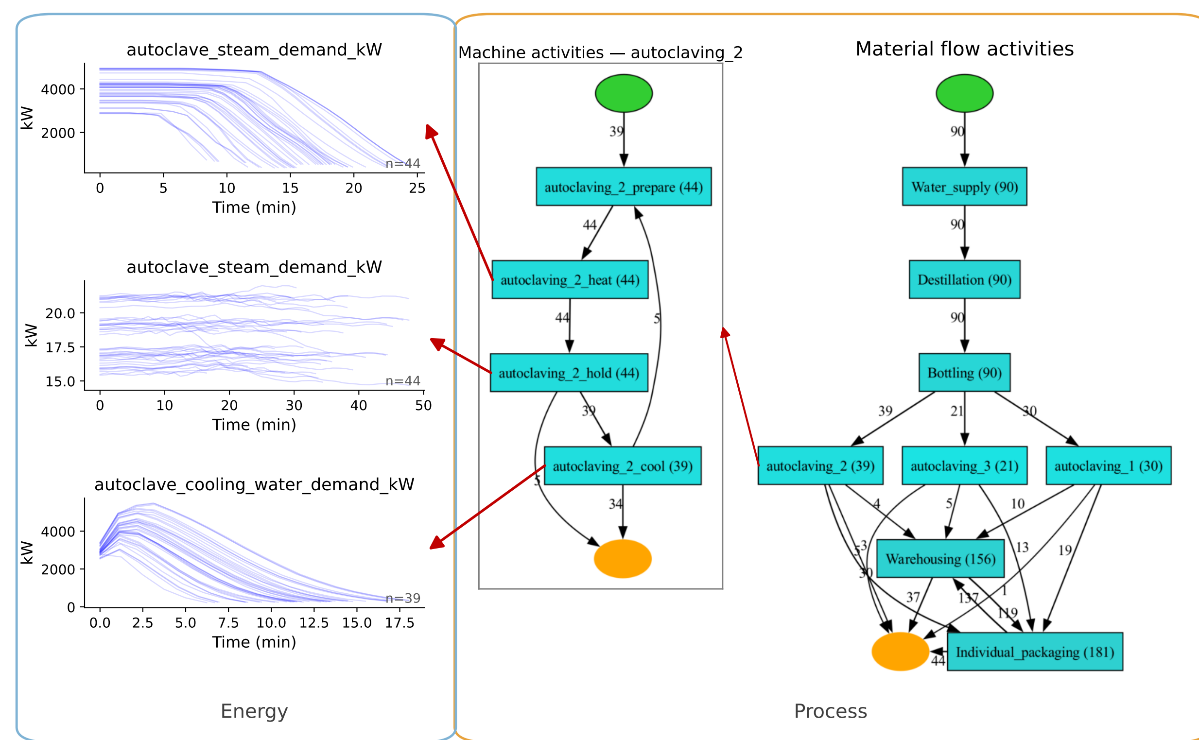
(b) simulated process and energy profiles
