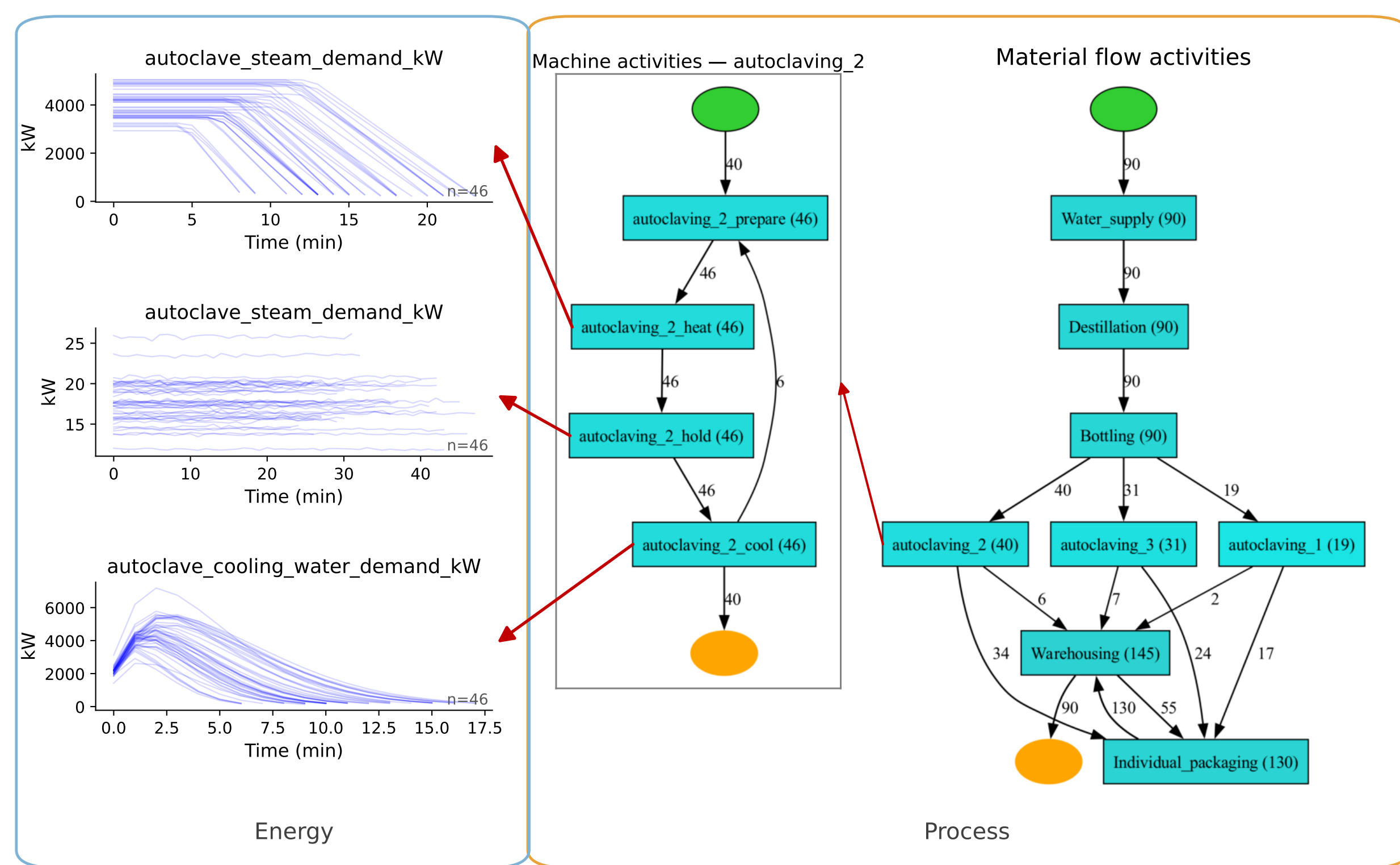
(a) real test set process and energy profiles
