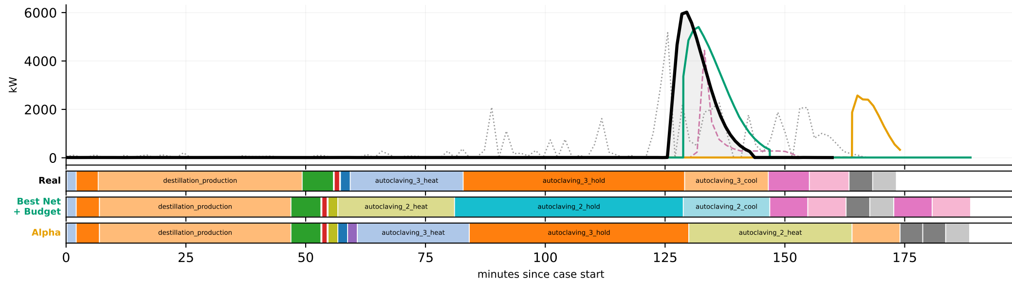
Autoclave cooling water demand — case batch_220
