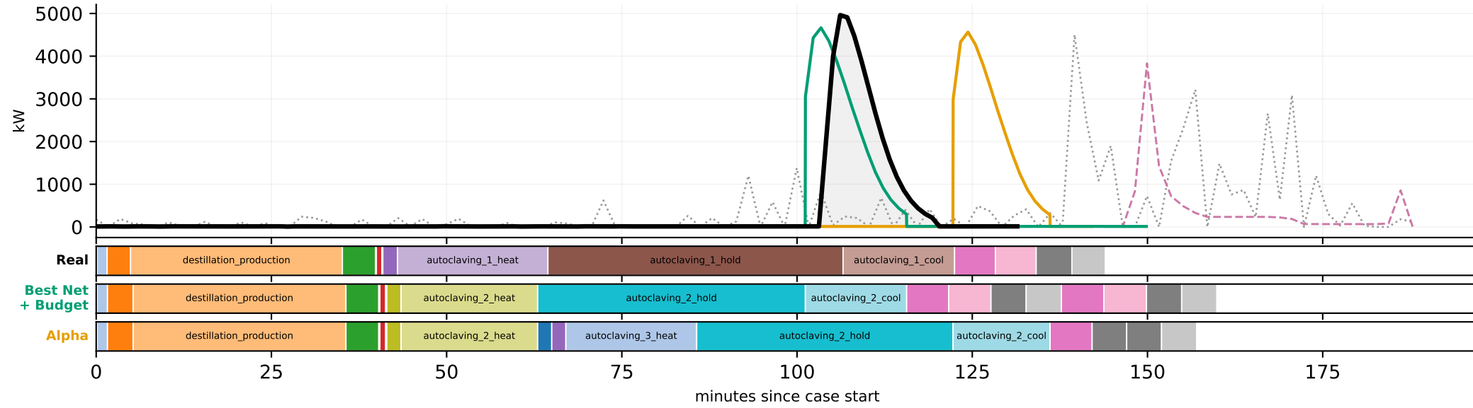
Autoclave cooling water demand — case batch_272
