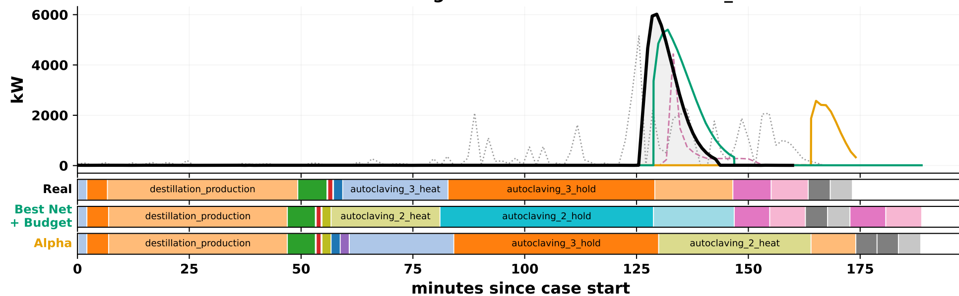
Autoclave cooling water demand — case batch_220
