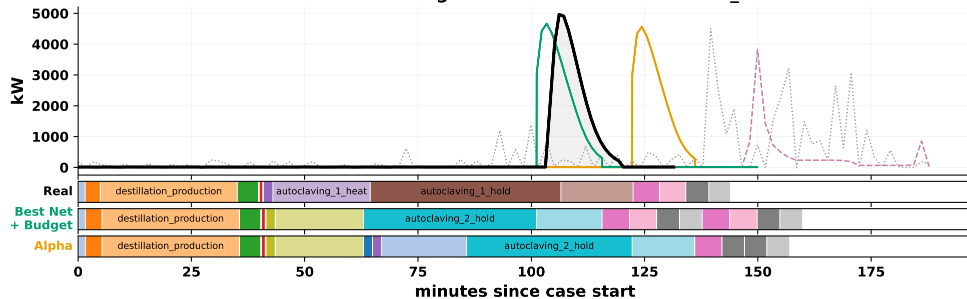
Autoclave cooling water demand — case batch_272
