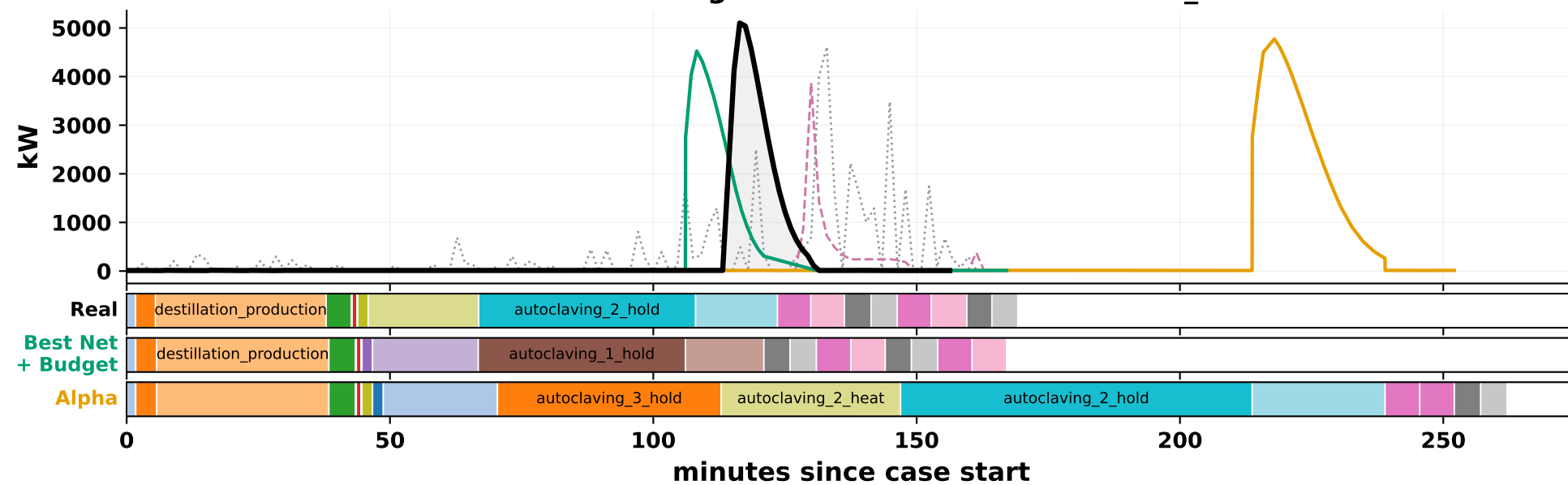
Autoclave cooling water demand — case batch_224
