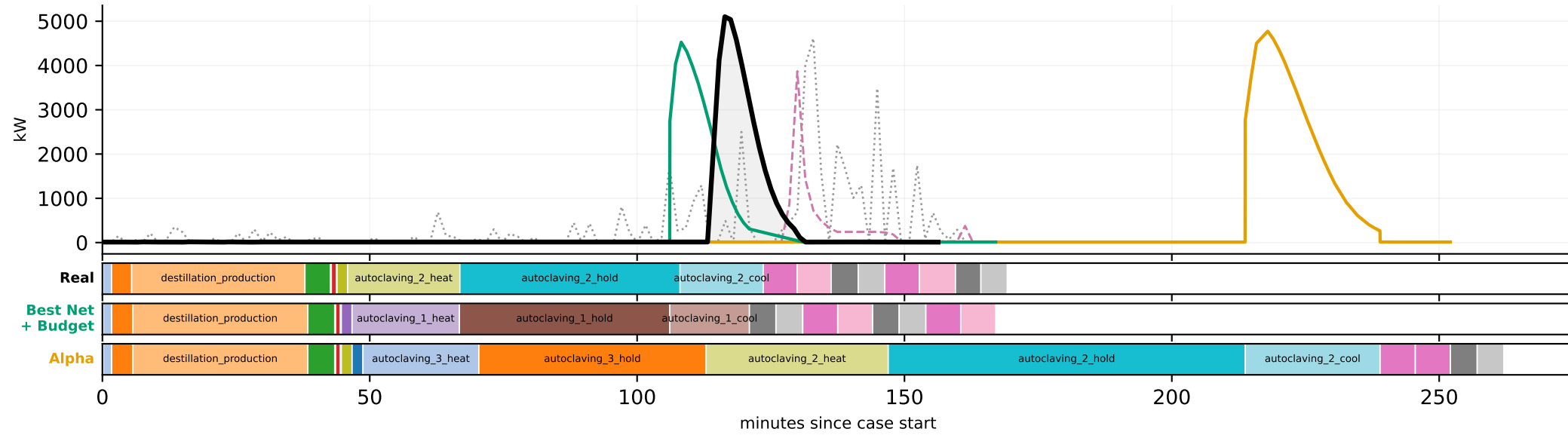
Autoclave cooling water demand — case batch_224
