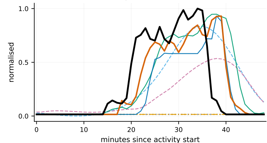
(15) Sensor 6 — Activity 23 curve 1, 49 points · realism 0.157
