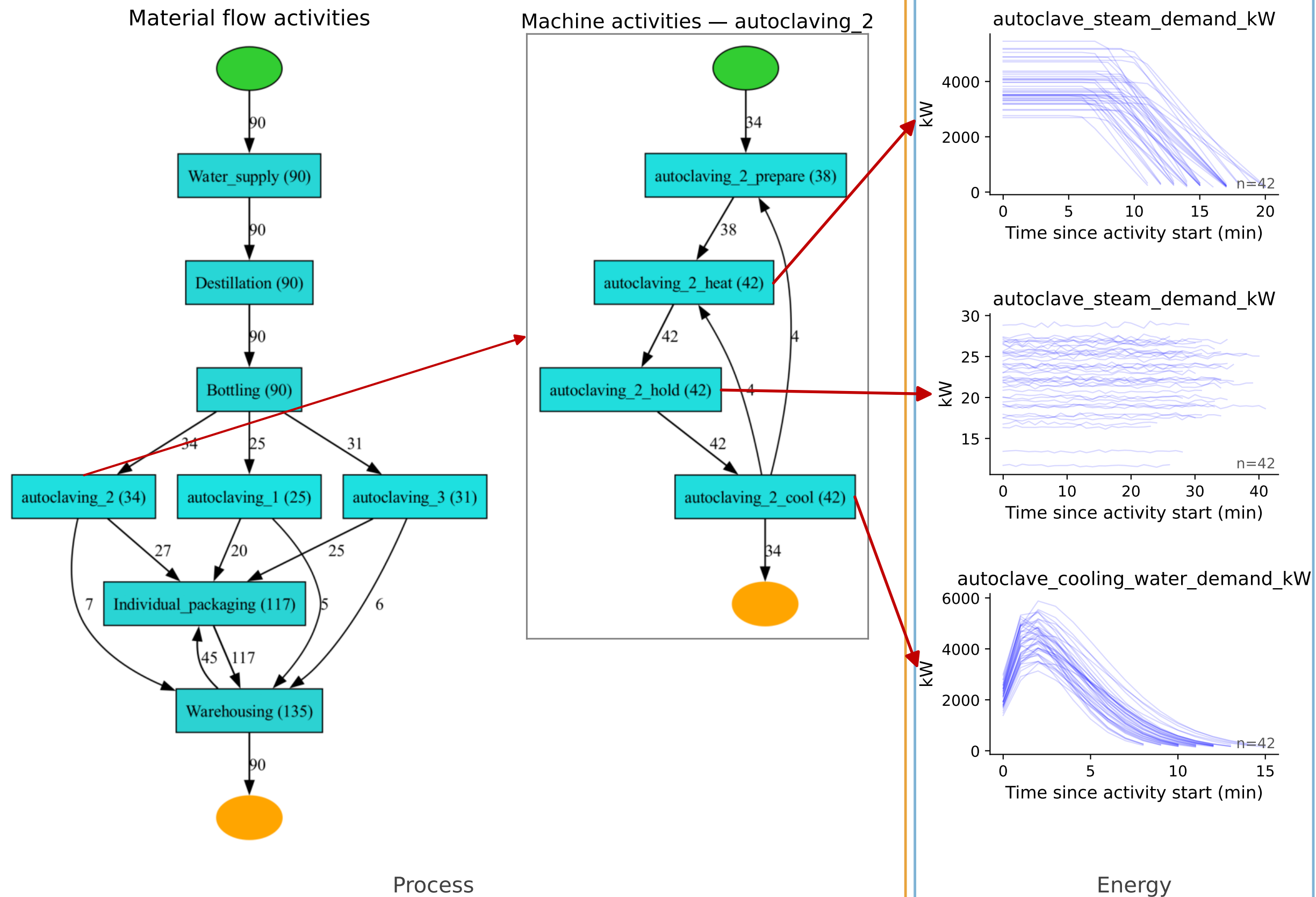
(a) real test set process and energy profiles
