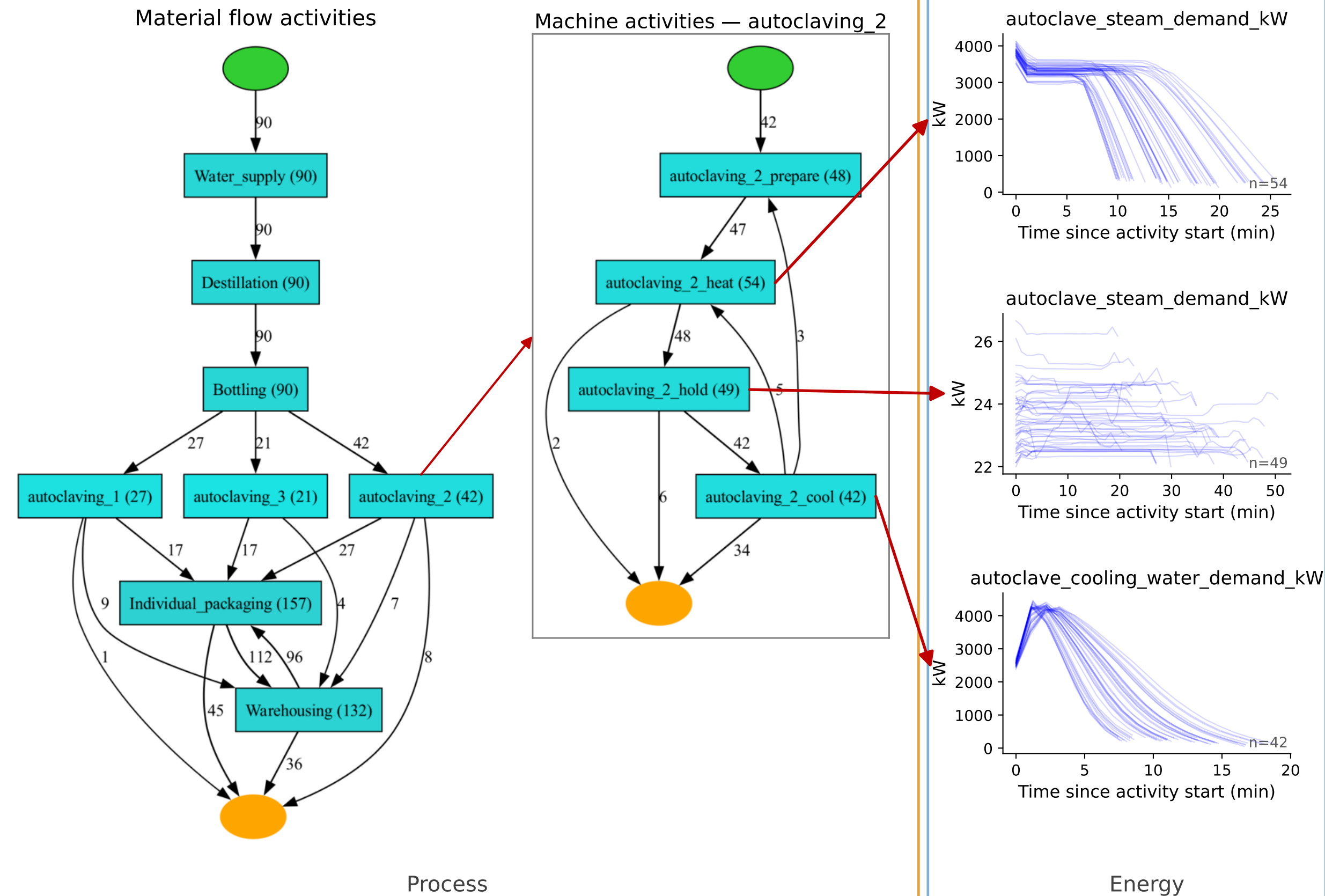
(b) simulated process and energy profiles
