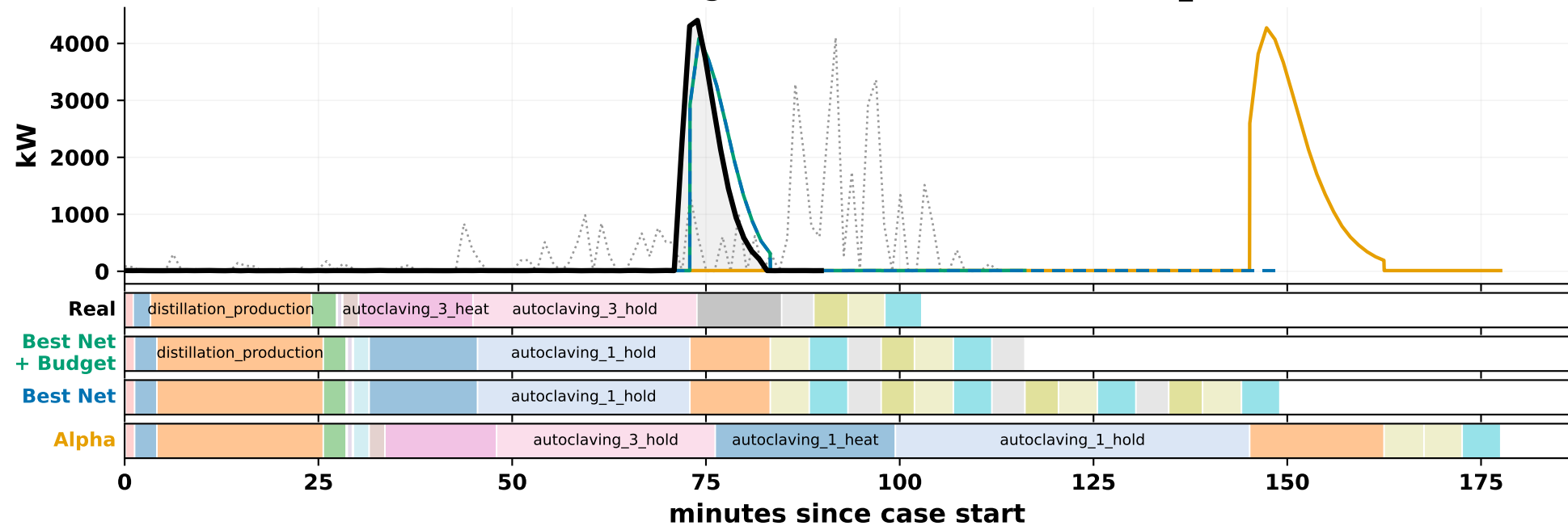
Autoclave cooling water demand — case batch_255
