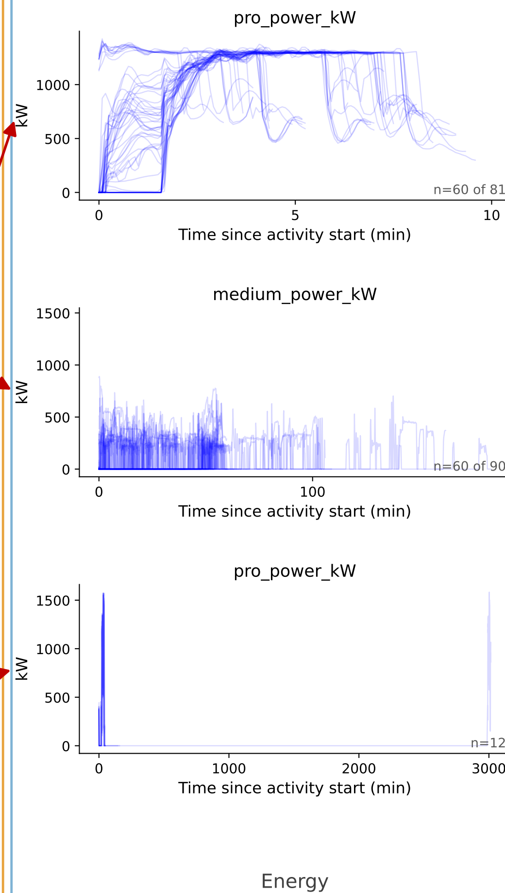
(a) real test set process and energy profiles — process_2 / I01
