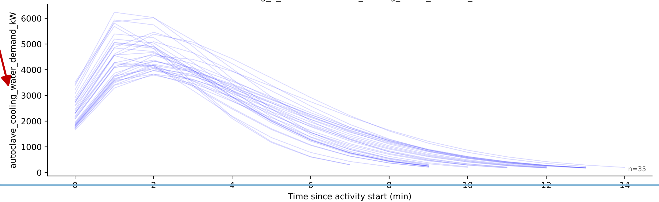
autoclaving_3_cool — autoclave_cooling_water_demand_kW
