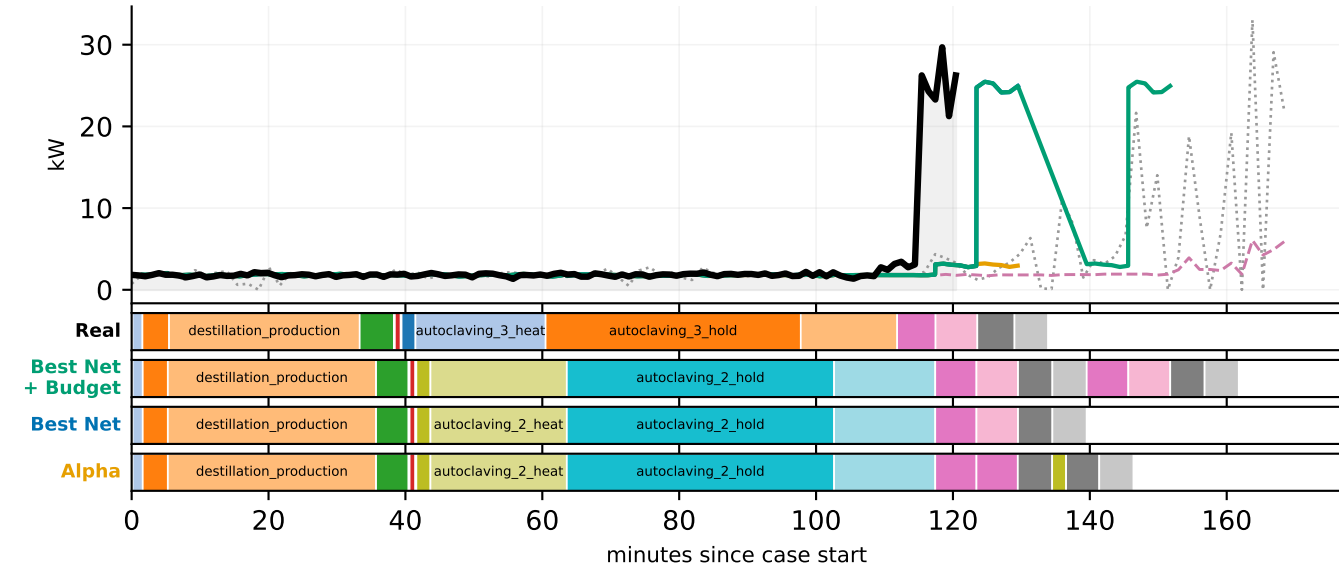
Power — individual packaging — case batch_261
