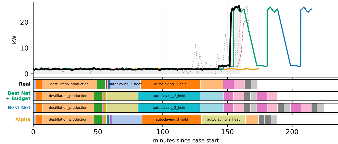
Power — individual packaging — case batch_220
