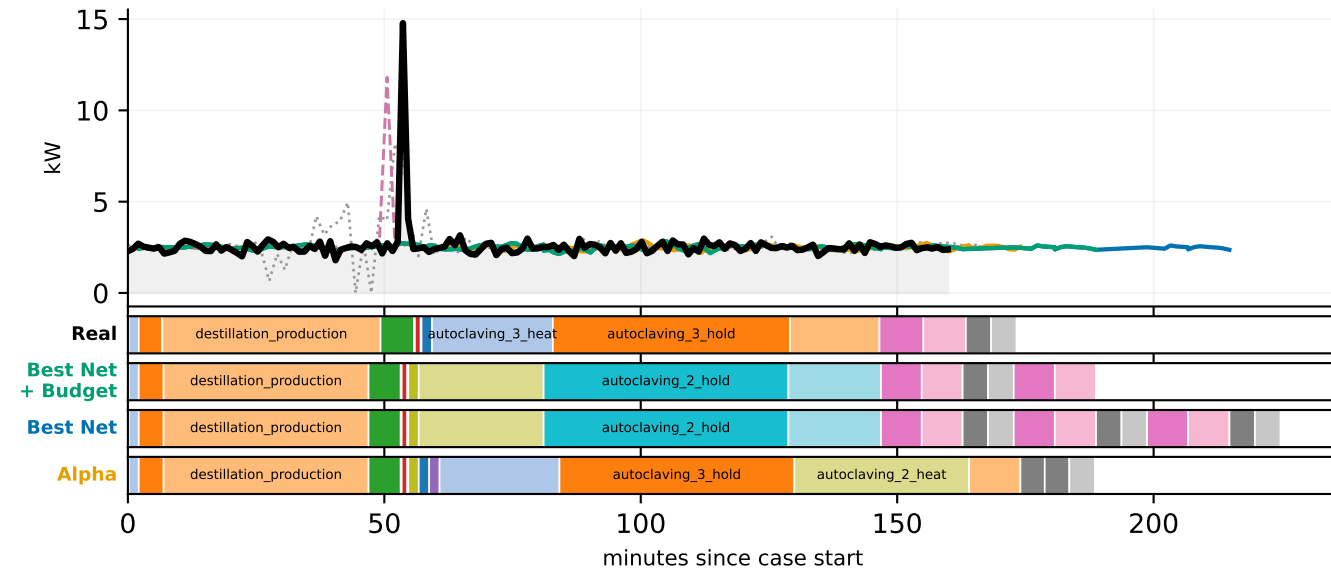
Power — bottling — case batch_220
