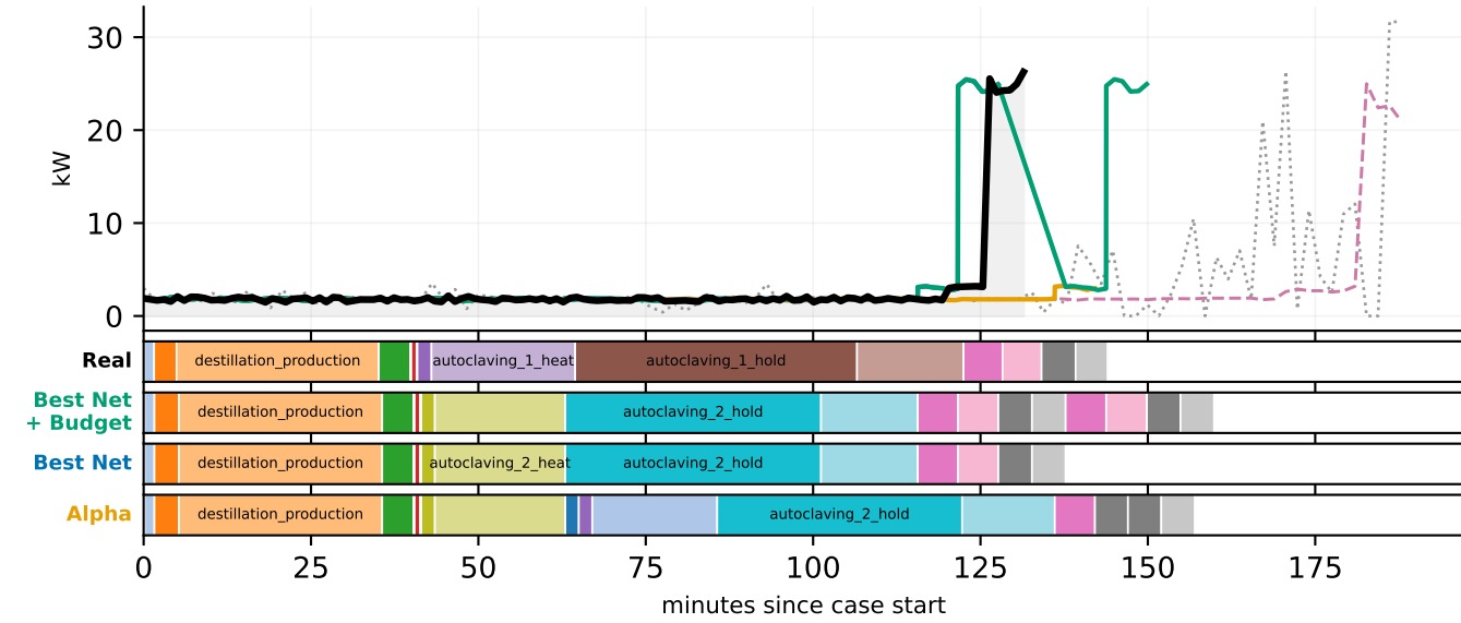
Power — individual packaging — case batch_272
