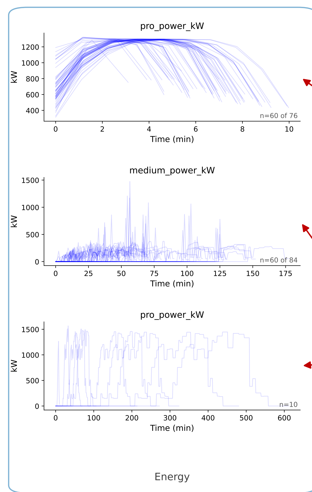
(b) simulated process and energy profiles — process_2 / I01
