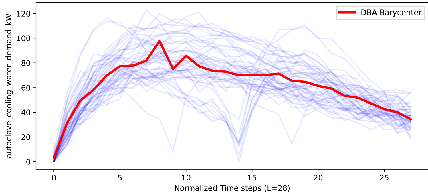
autoclaving_2_cool - autoclave_cooling_water_demand_kW (DBA)
