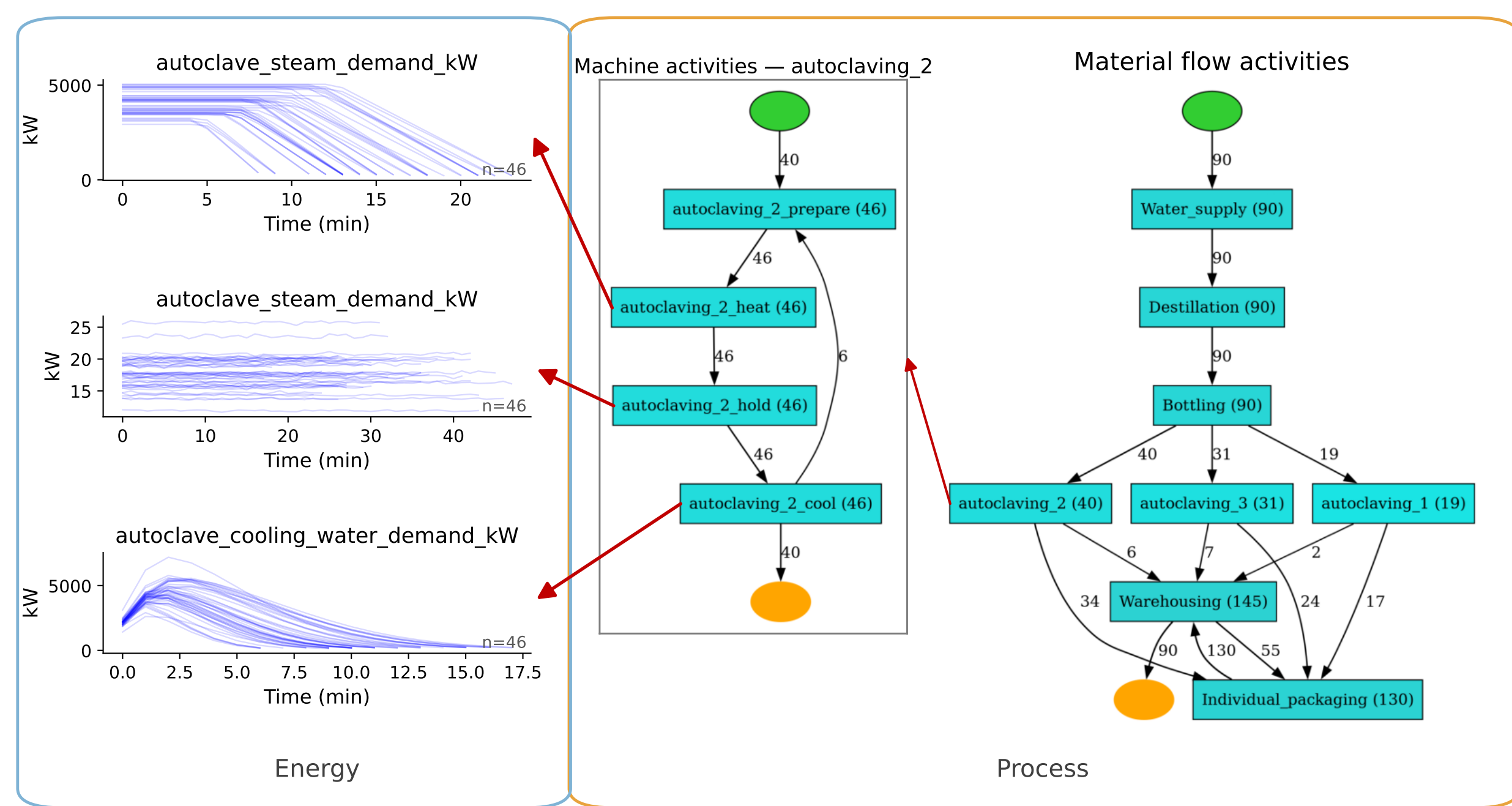
(a) real test set process and energy profiles
