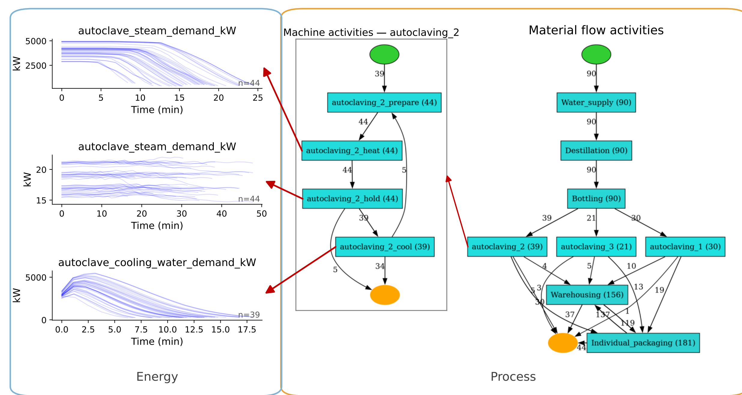
(b) simulated process and energy profiles
