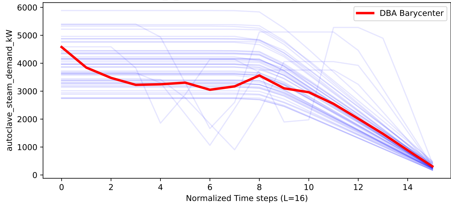
autoclaving_2_heat - autoclave_steam_demand_kW (DBA)
