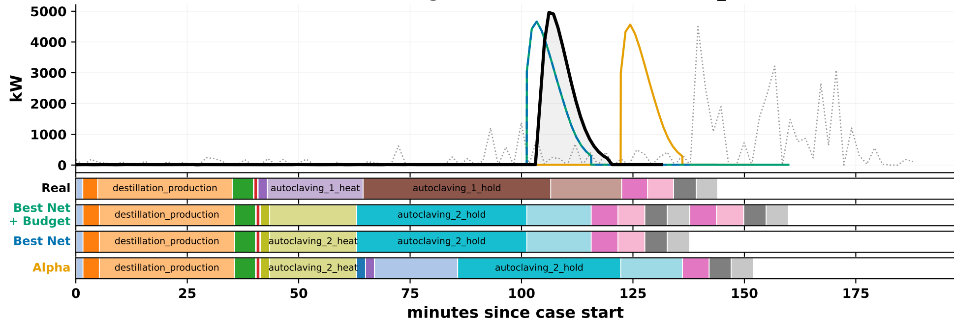
Autoclave cooling water demand — case batch_272
