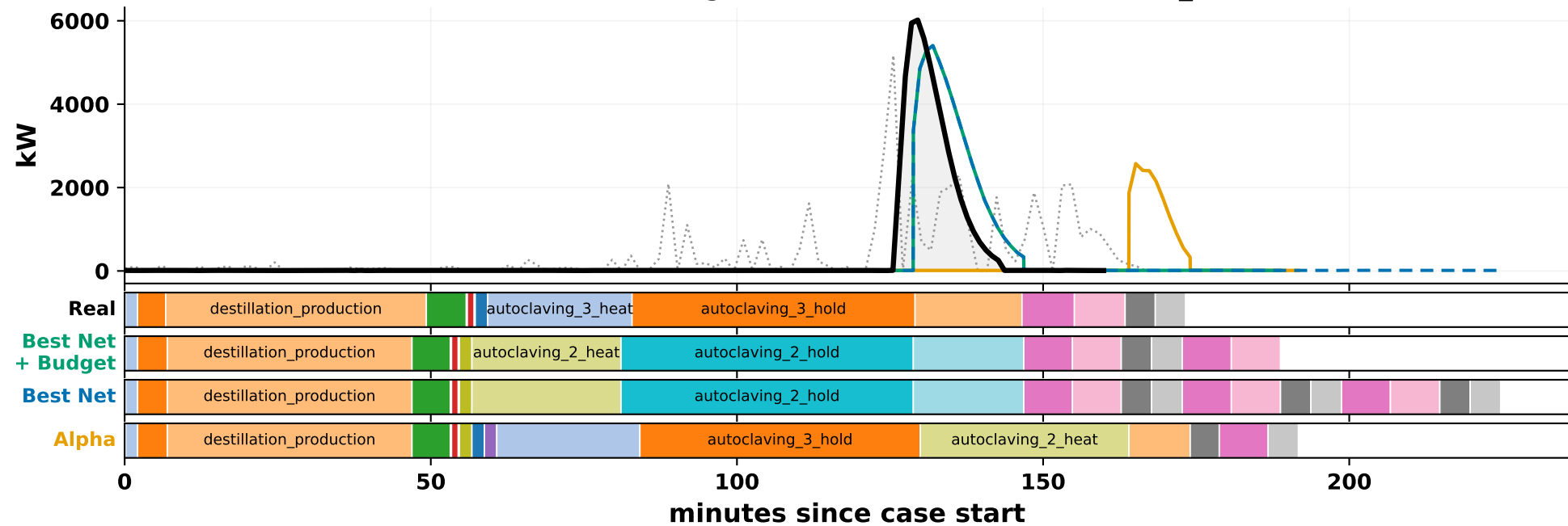
Autoclave cooling water demand — case batch_220
