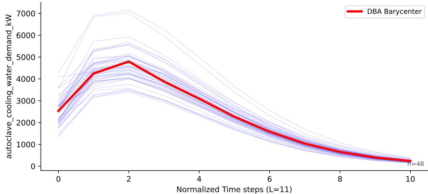
autoclaving_2_cool — autoclave_cooling_water_demand_kW (real (gold expanded))
