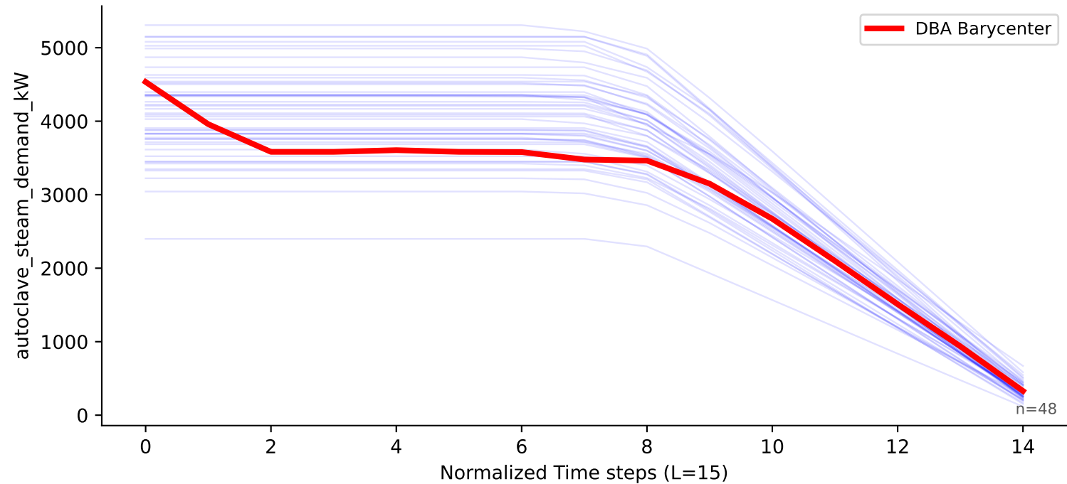
autoclaving_2_heat — autoclave_steam_demand_kW (real (gold expanded))
