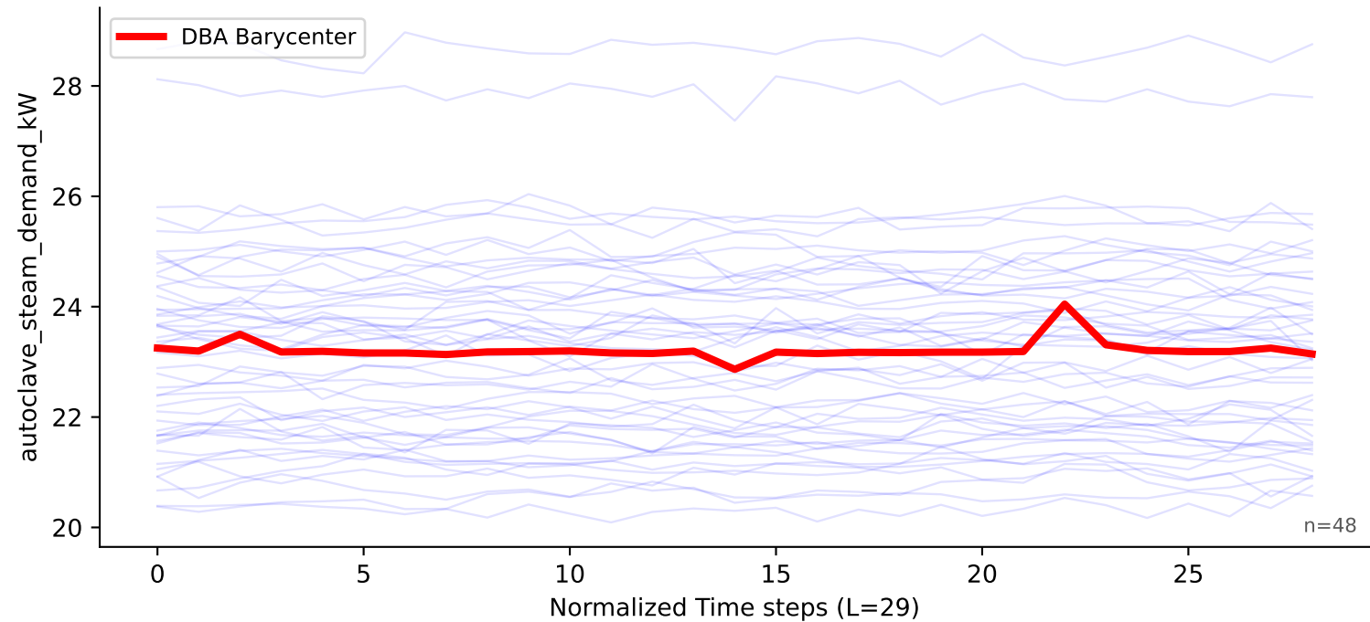
autoclaving_2_hold — autoclave_steam_demand_kW (real (gold expanded))
