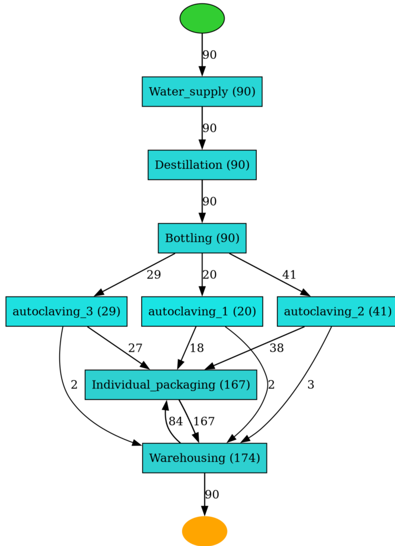
Material flow — stations, Autoclaving split into machines
