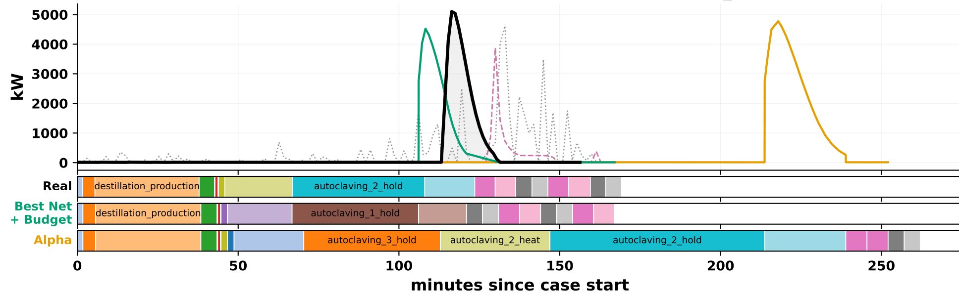
Autoclave cooling water demand — case batch_224
