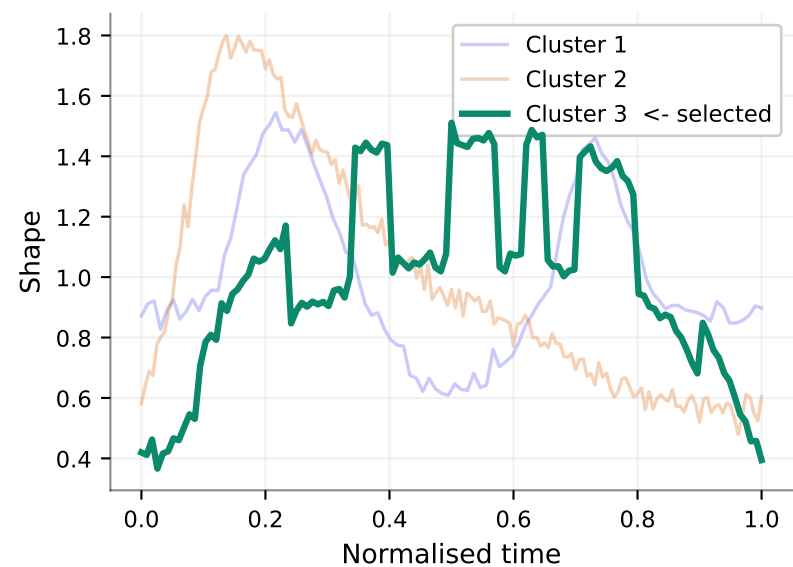
(d) Shape classifier picks a cluster from attributes + ef_* , one row per curve
